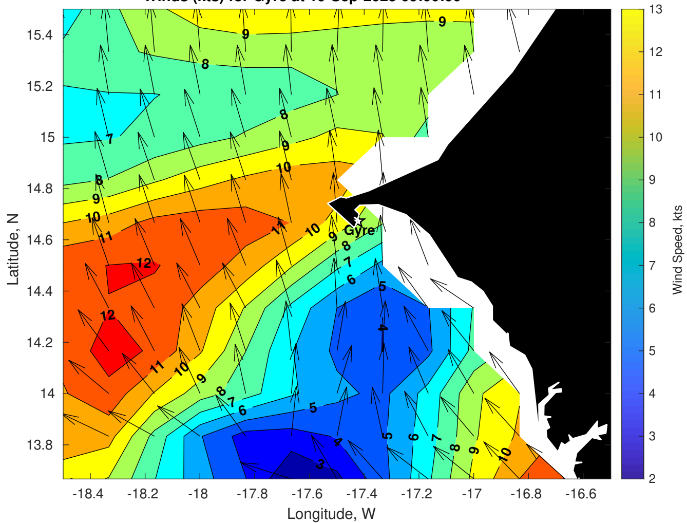
Winds (kts) for Gyre at 19-Sep-2025 09:00:00
