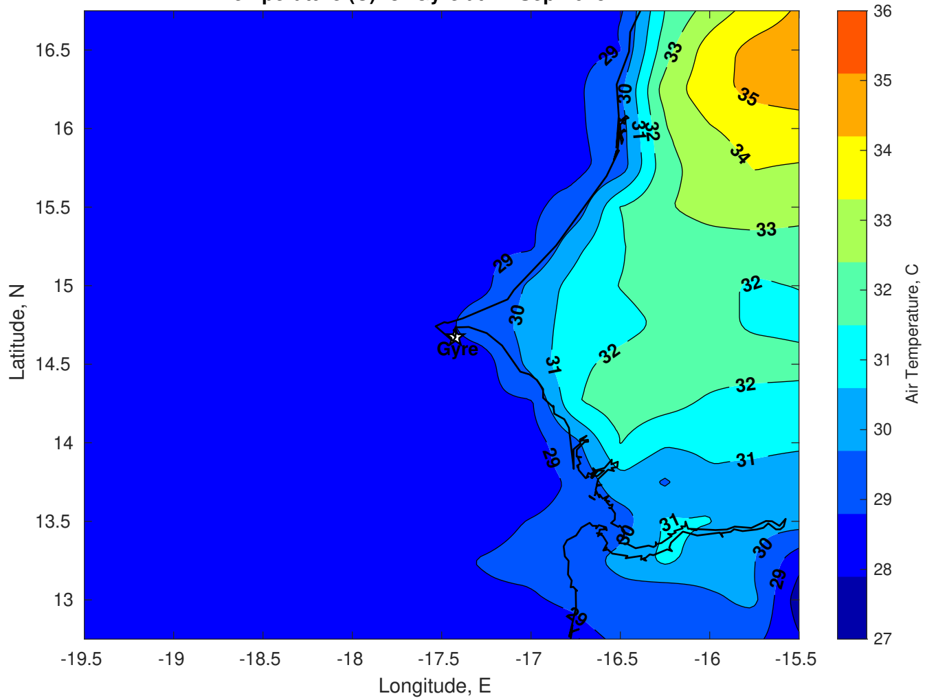
Air Temperature (C) for Gyre at 17-Sep-2025
