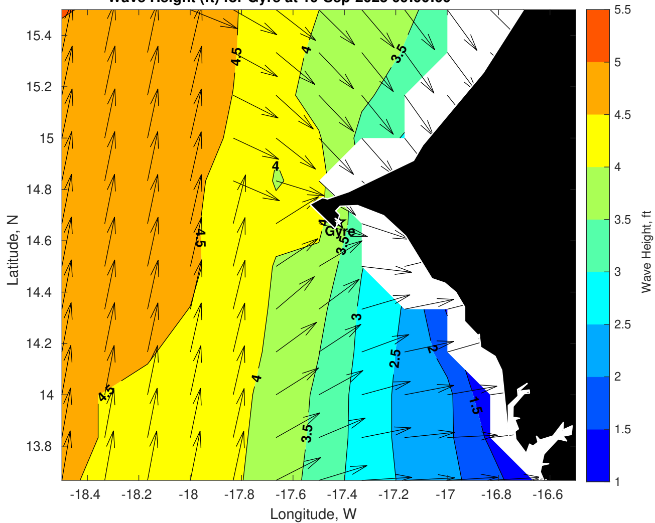
Wave Height (ft) for Gyre at 19-Sep-2025 09:00:00
