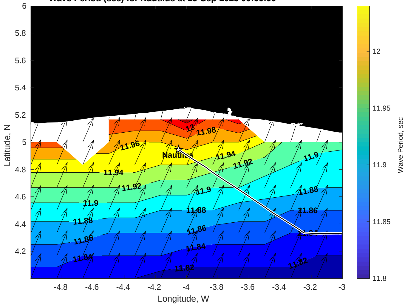
Wave Period (sec) for Nautilus at 19-Sep-2025 09:00:00
