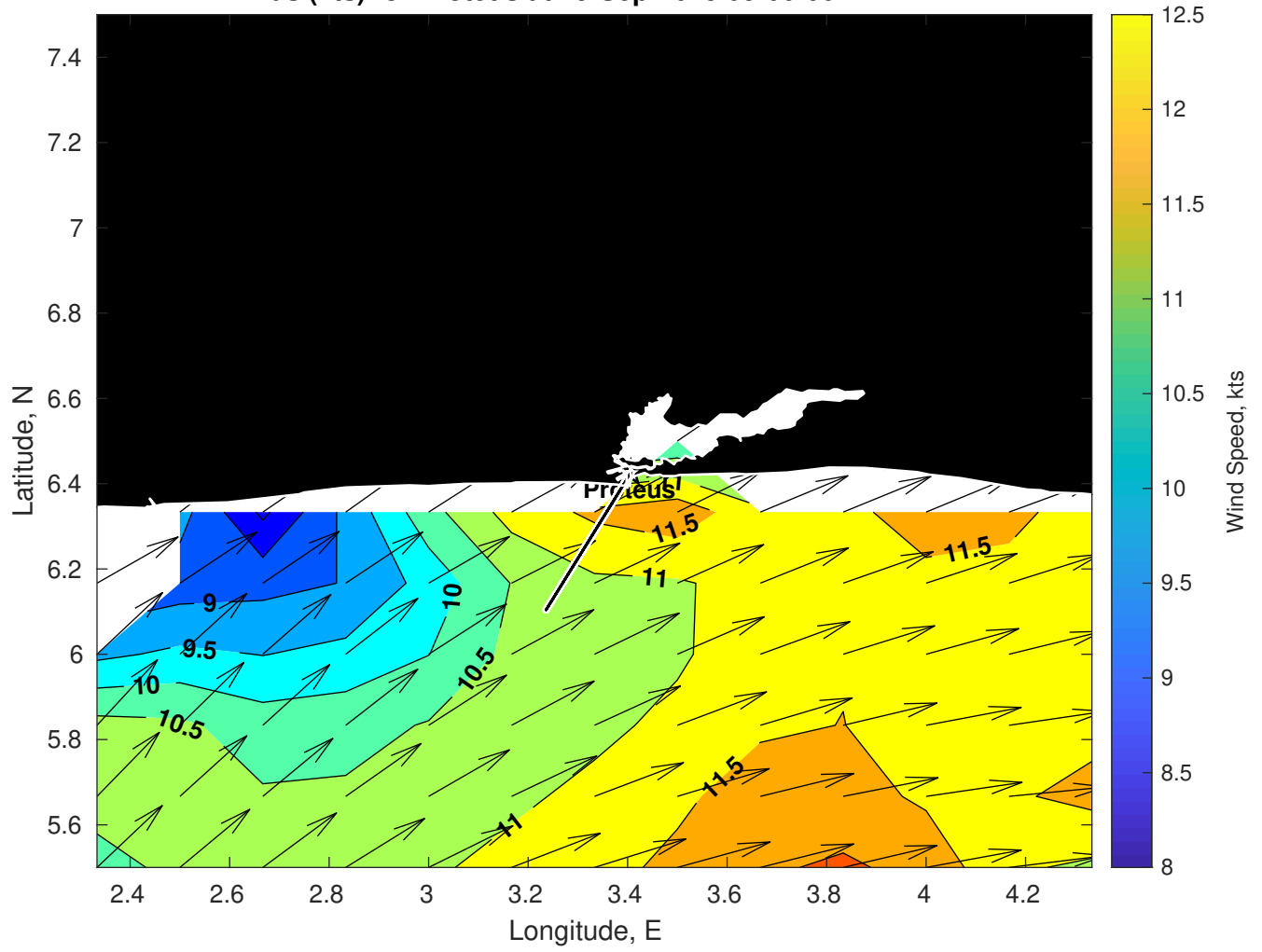
Winds (kts) for Proteus at 19-Sep-2025 09:00:00
