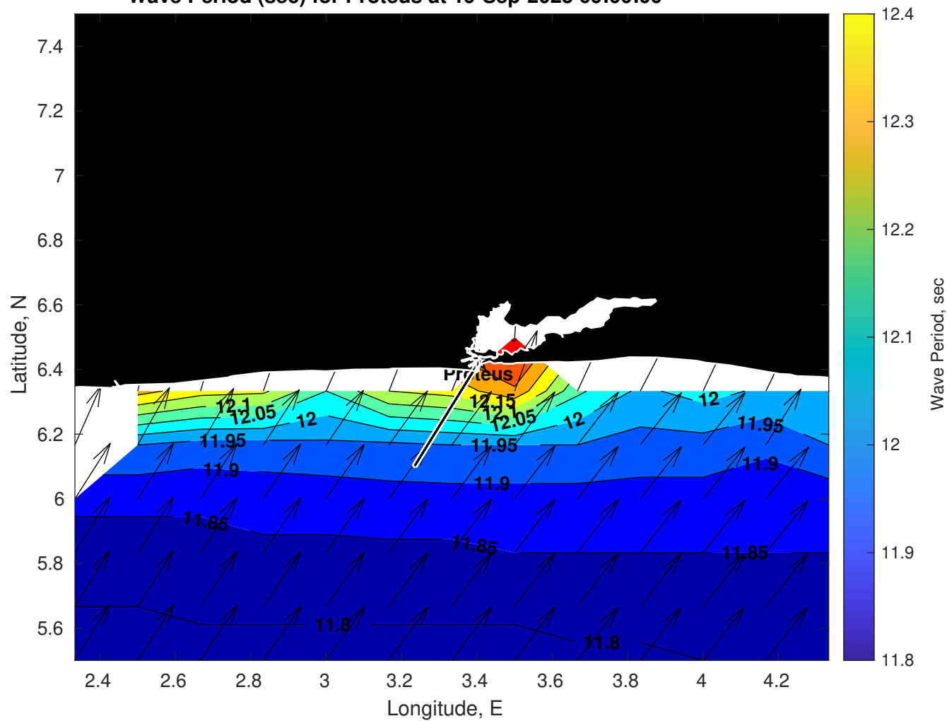
Wave Period (sec) for Proteus at 19-Sep-2025 09:00:00
