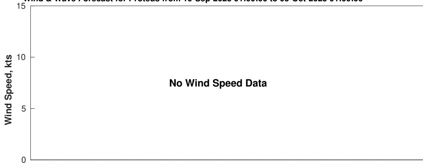
Wind & Wave Forecast for Proteus from 19-Sep-2025 01:00:00 to 05-Oct-2025 01:00:00
