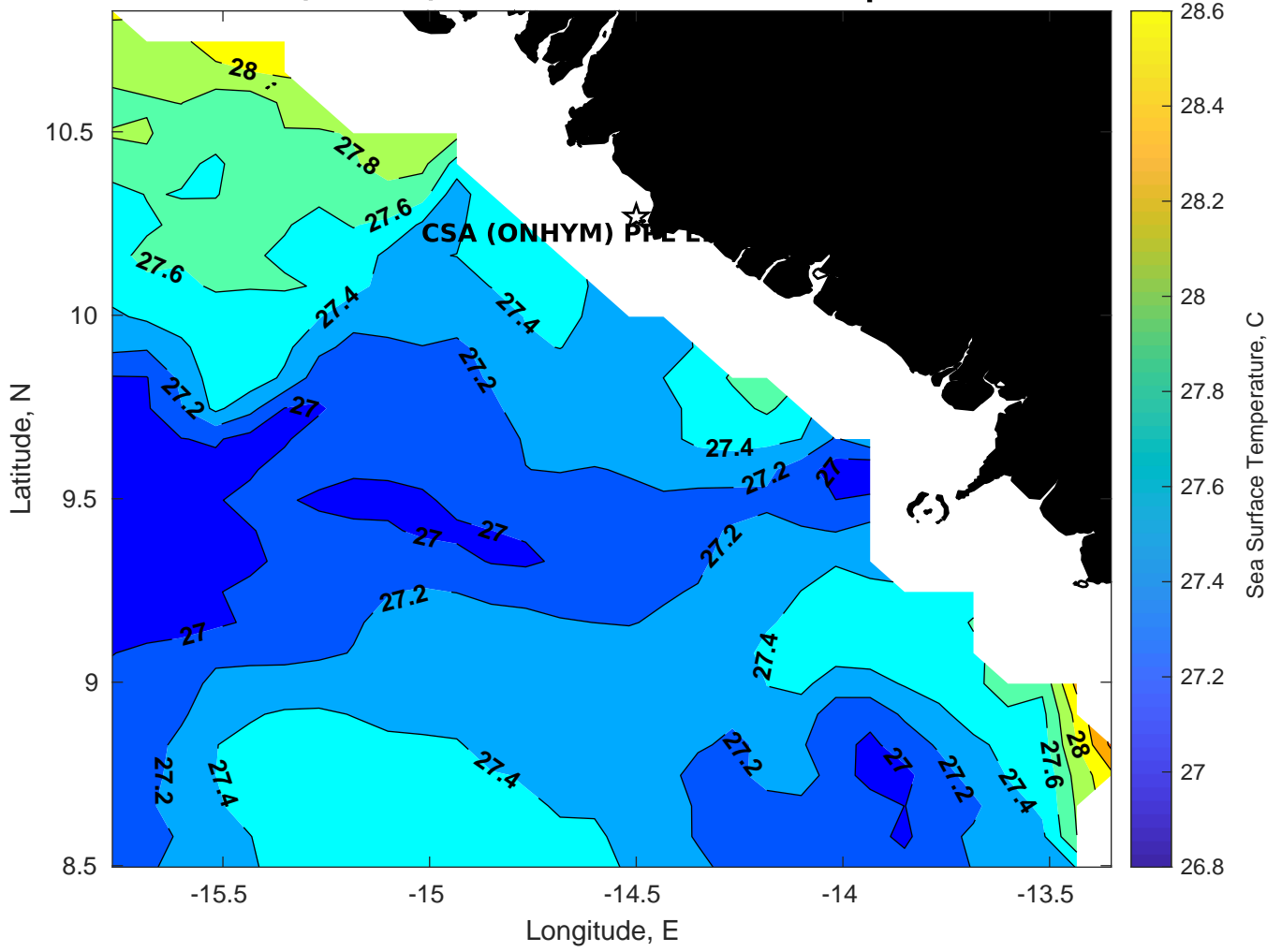
SST for CSA (ONHYM) PPL EBS - Guinea at 17-Sep-2025 00:00:00
