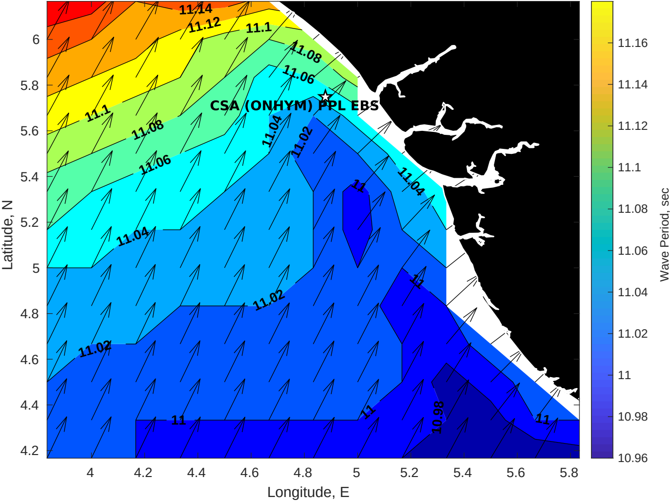
Wave Period (sec) for CSA (ONHYM) PPL EBS - Nigeria at 20-Sep-2025 09:00:00
