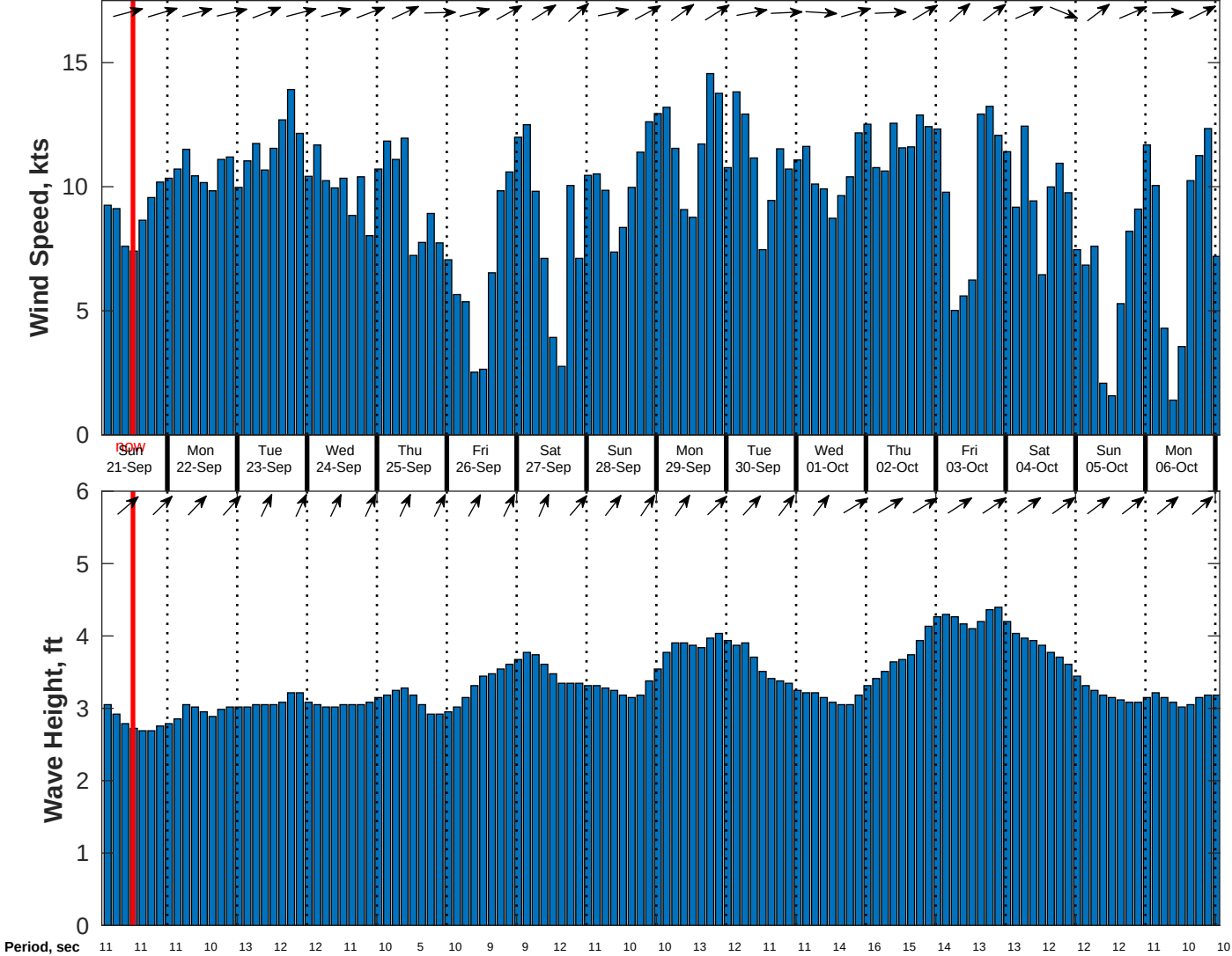
Wind & Wave Forecast for CSA (ONHYM) PPL EBS - Nigeria from 20-Sep-2025 02:00:00 to 06-Oct-2025 02:00:00
