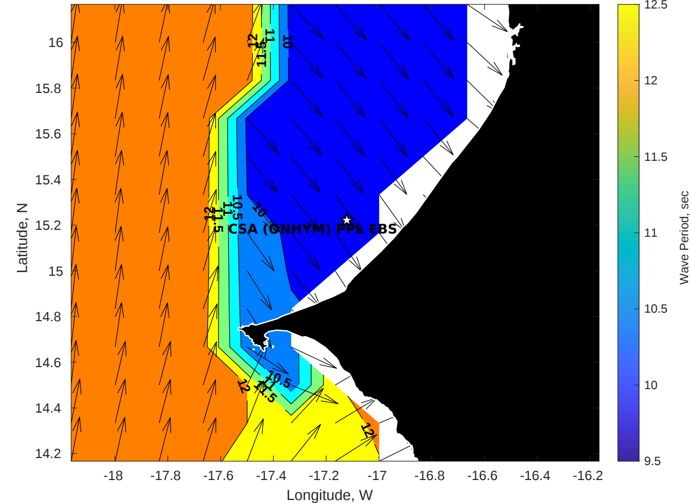
Wave Period (sec) for CSA (ONHYM) PPL EBS - Senegal at 20-Sep-2025 09:00:00
