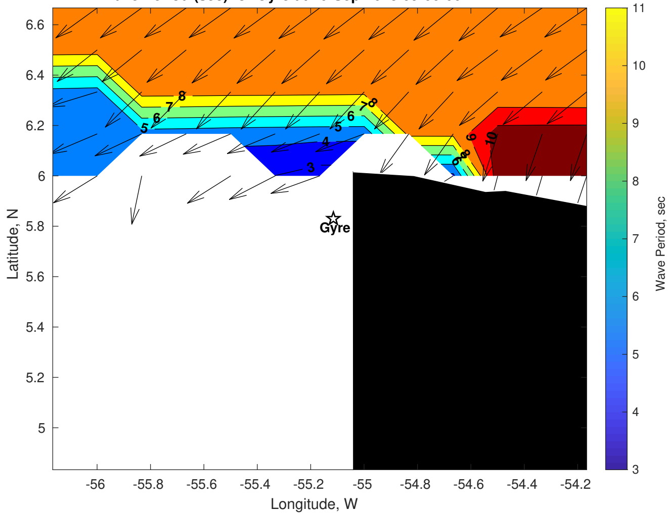
Wave Period (sec) for Gyre at 20-Sep-2025 09:00:00
