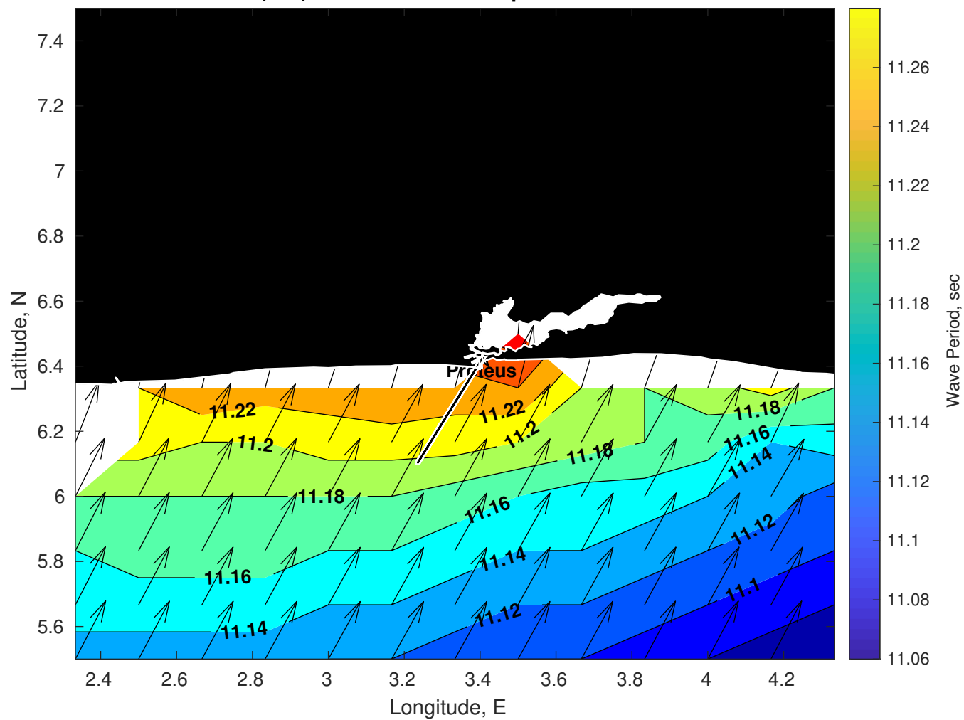
Wave Period (sec) for Proteus at 20-Sep-2025 09:00:00
