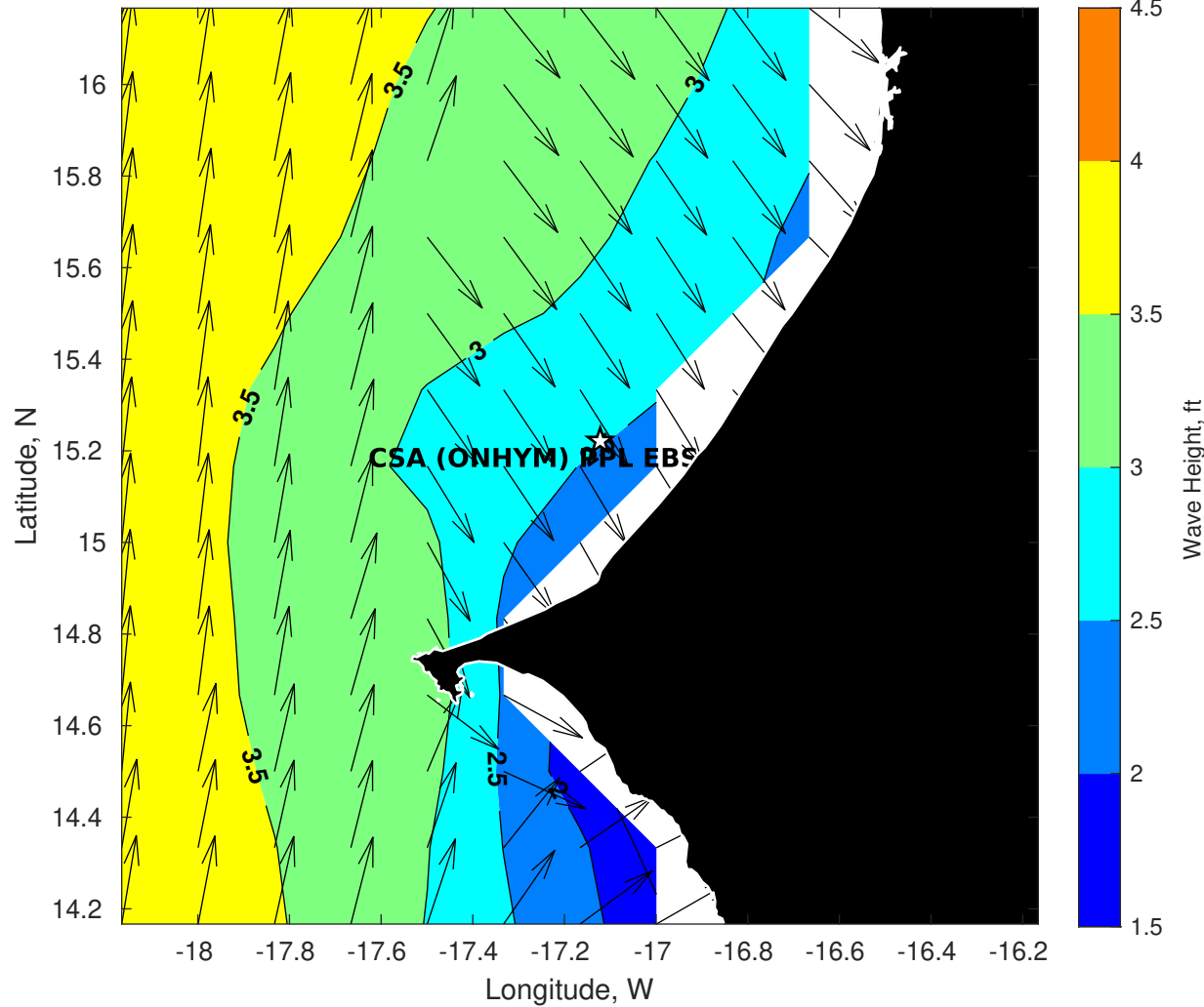
Wave Height (ft) for CSA (ONHYM) PPL EBS - Senegal at 20-Sep-2025 09:00:00
