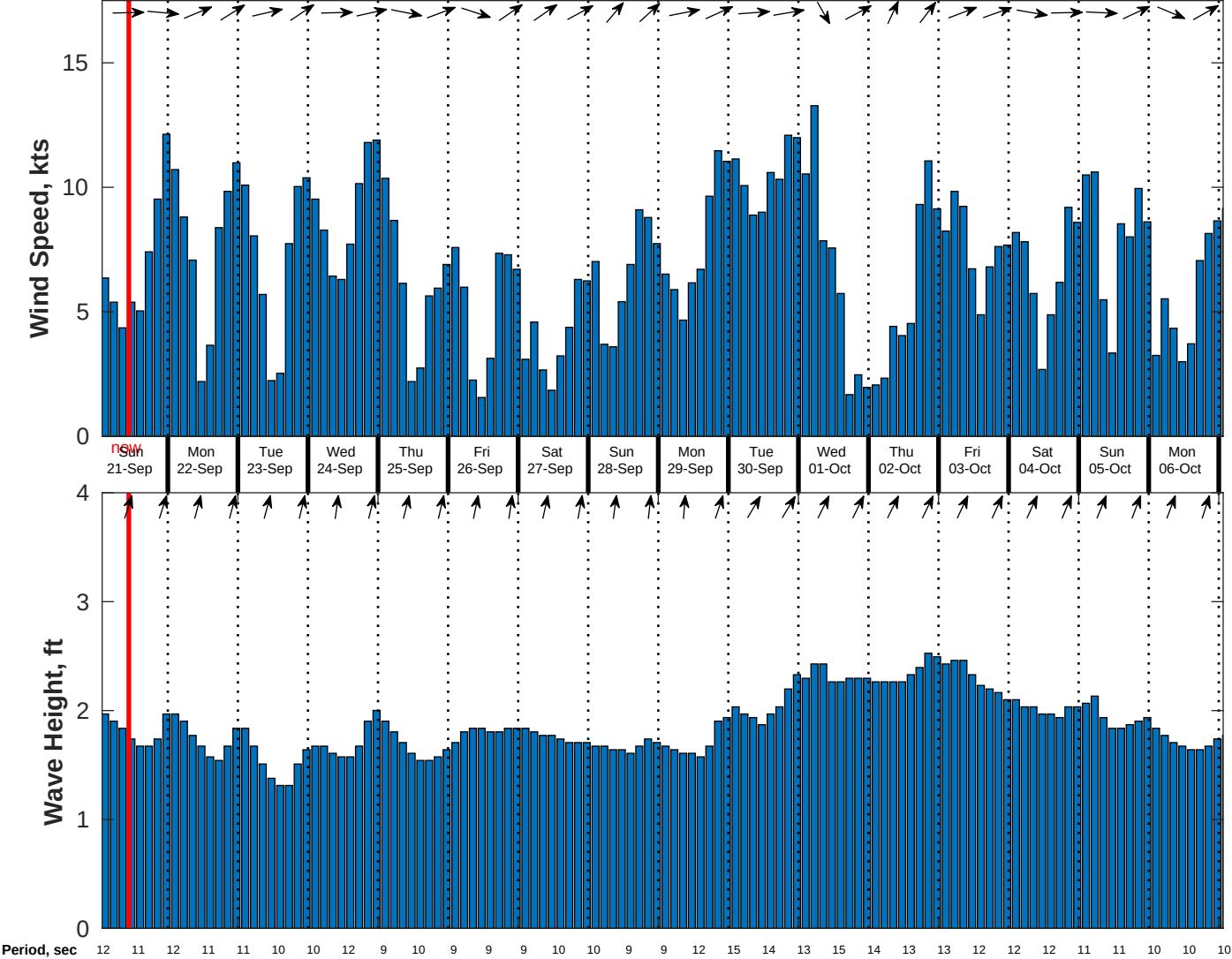
Wind & Wave Forecast for CSA (ONHYM) PPL EBS - Sierra Leone from 20-Sep-2025 01:00:00 to 06-Oct-2025 01:00:00
