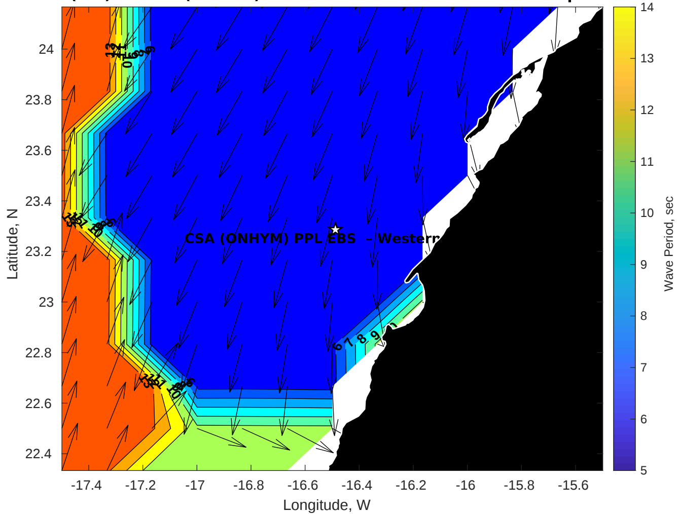
Wave Period (sec) for CSA (ONHYM) PPL EBS - Western Sahara at 20-Sep-2025 09:00:00
