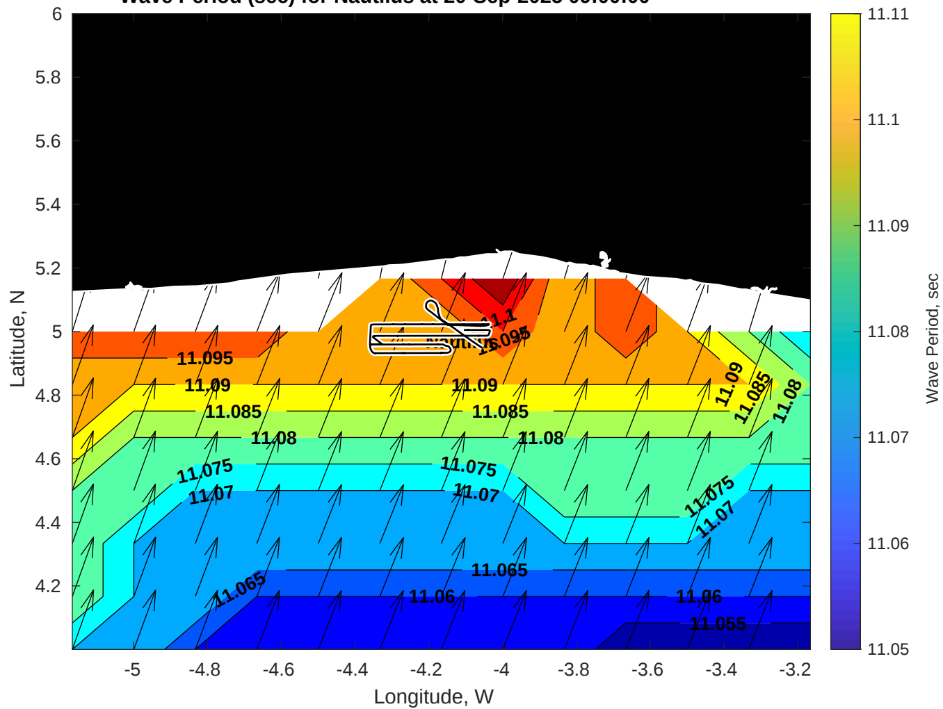
Wave Period (sec) for Nautilus at 20-Sep-2025 09:00:00
