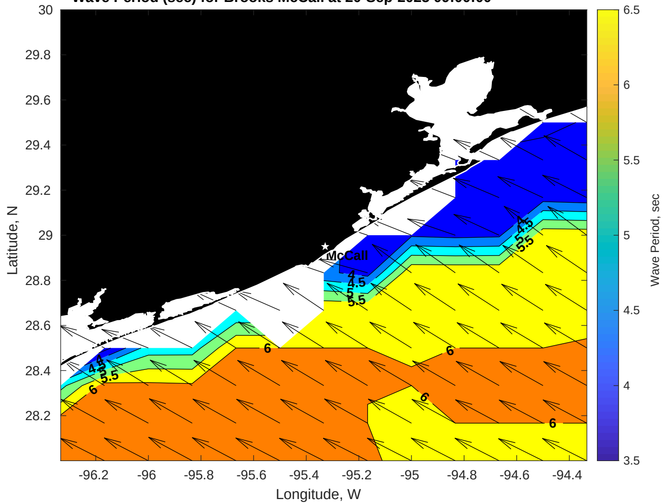
Wave Period (sec) for Brooks McCall at 20-Sep-2025 09:00:00
