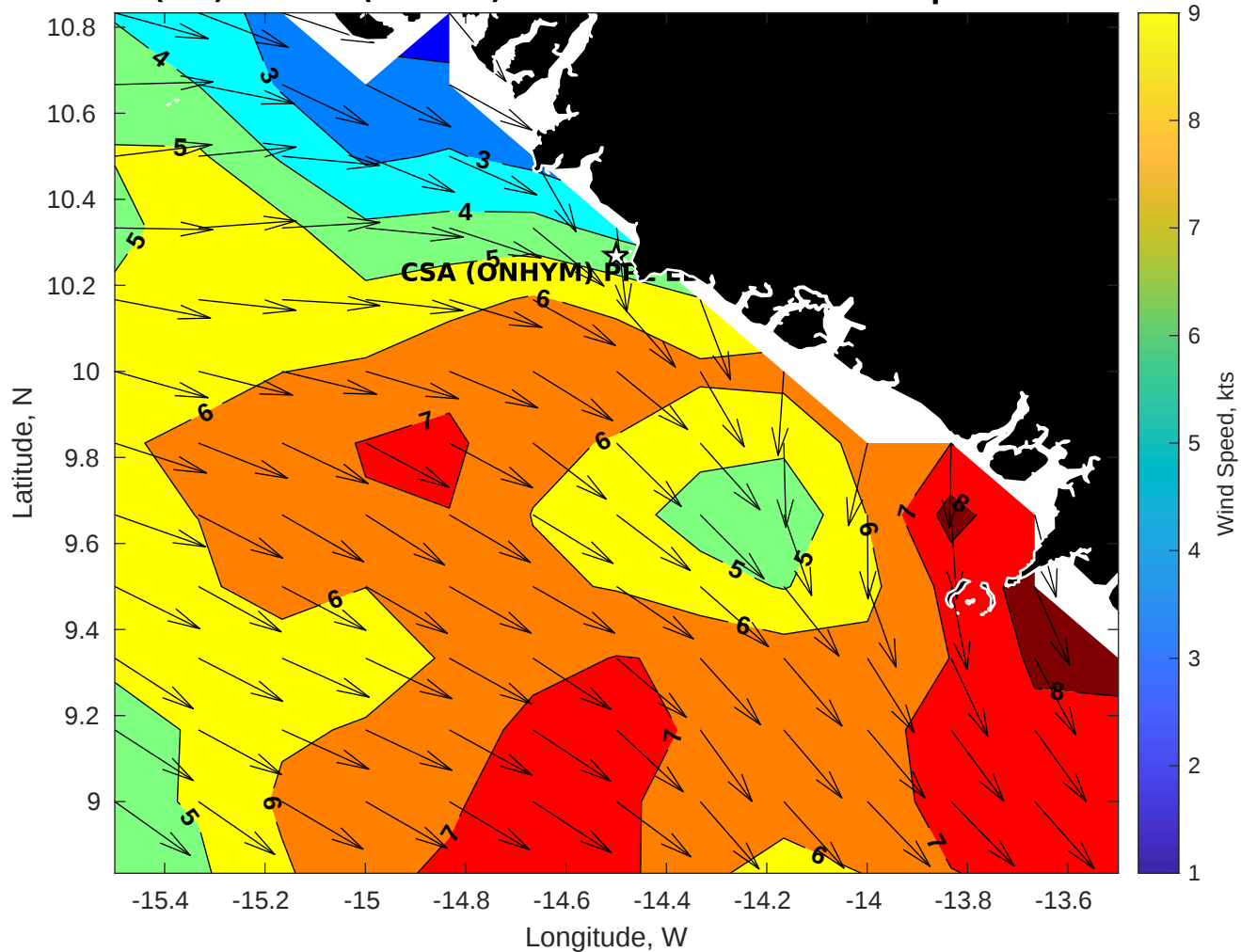
Winds (kts) for CSA (ONHYM) PPL EBS - Guinea at 20-Sep-2025 09:00:00
