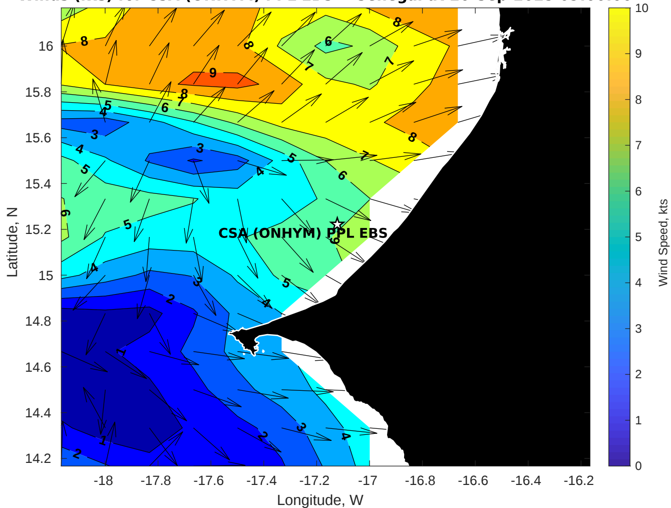
Winds (kts) for CSA (ONHYM) PPL EBS - Senegal at 20-Sep-2025 09:00:00
