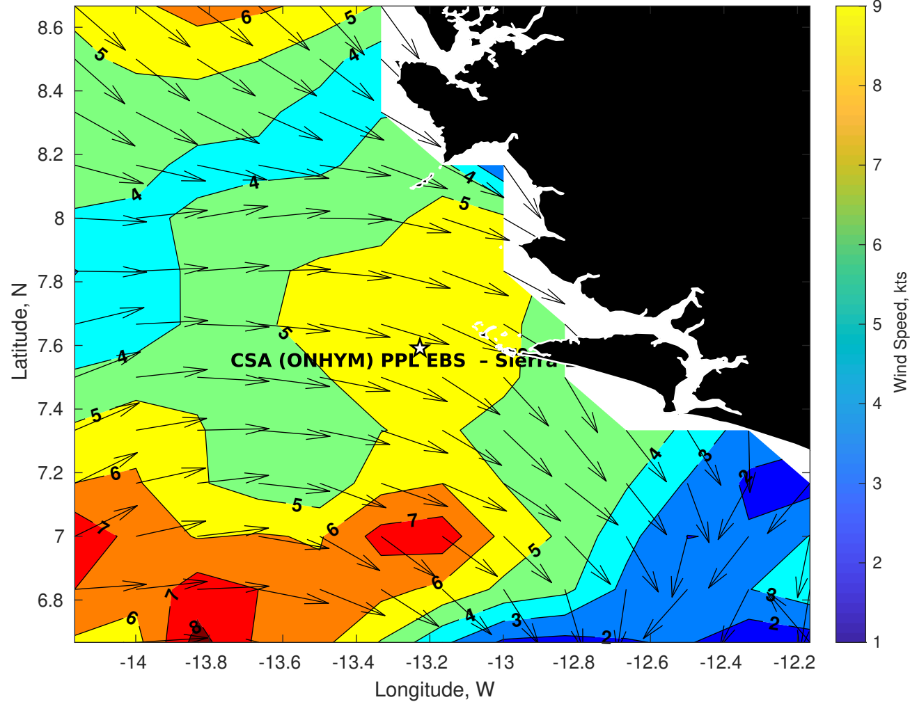
Winds (kts) for CSA (ONHYM) PPL EBS - Sierra Leone at 20-Sep-2025 09:00:00
