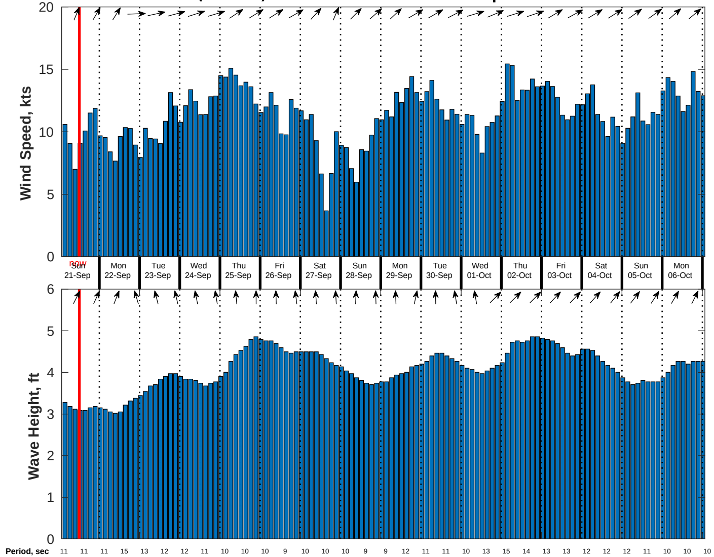
Wind & Wave Forecast for CSA (ONHYM) PPL EBS - Ghana from 20-Sep-2025 02:00:00 to 06-Oct-2025 02:00:00
