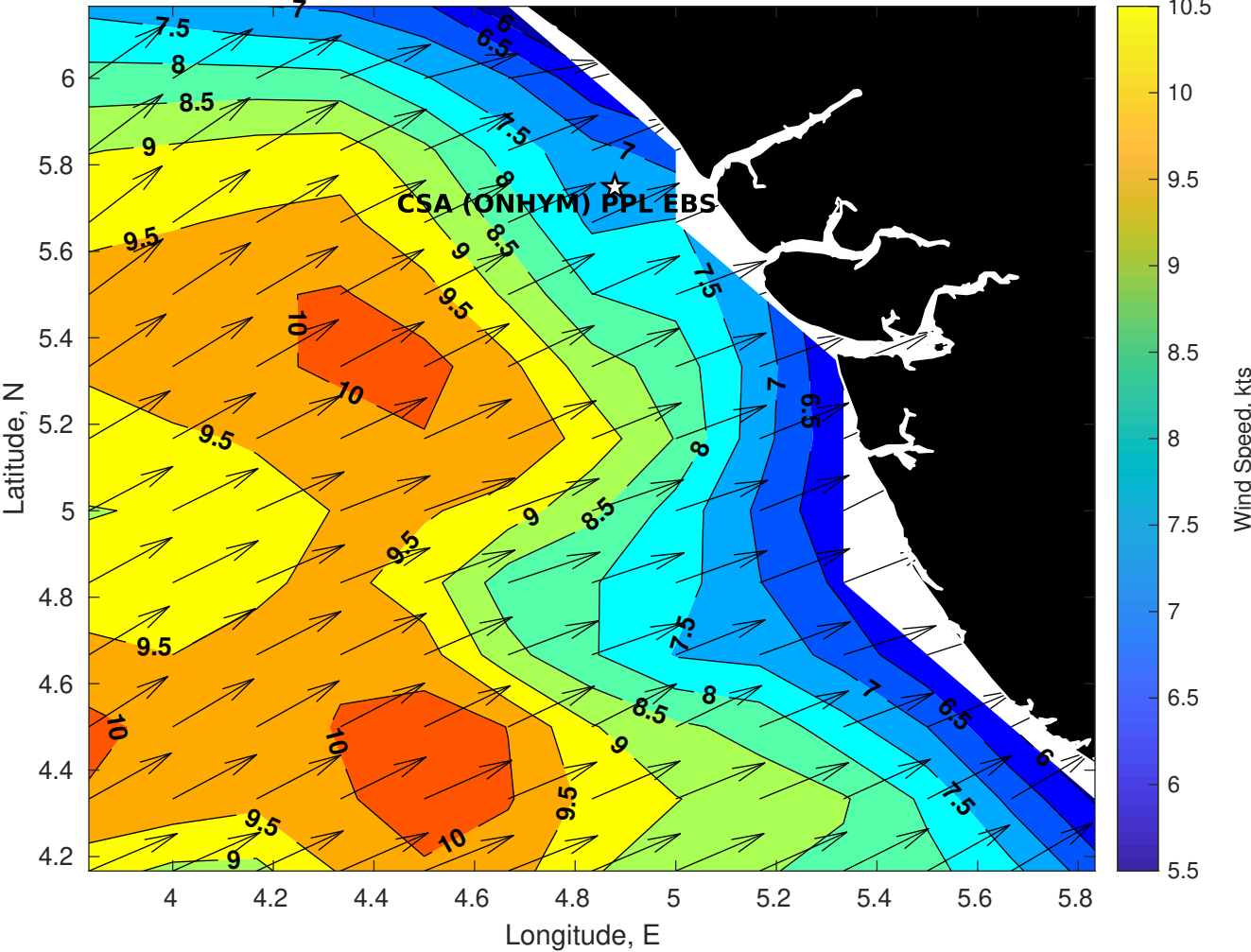
Winds (kts) for CSA (ONHYM) PPL EBS - Nigeria at 20-Sep-2025 09:00:00
