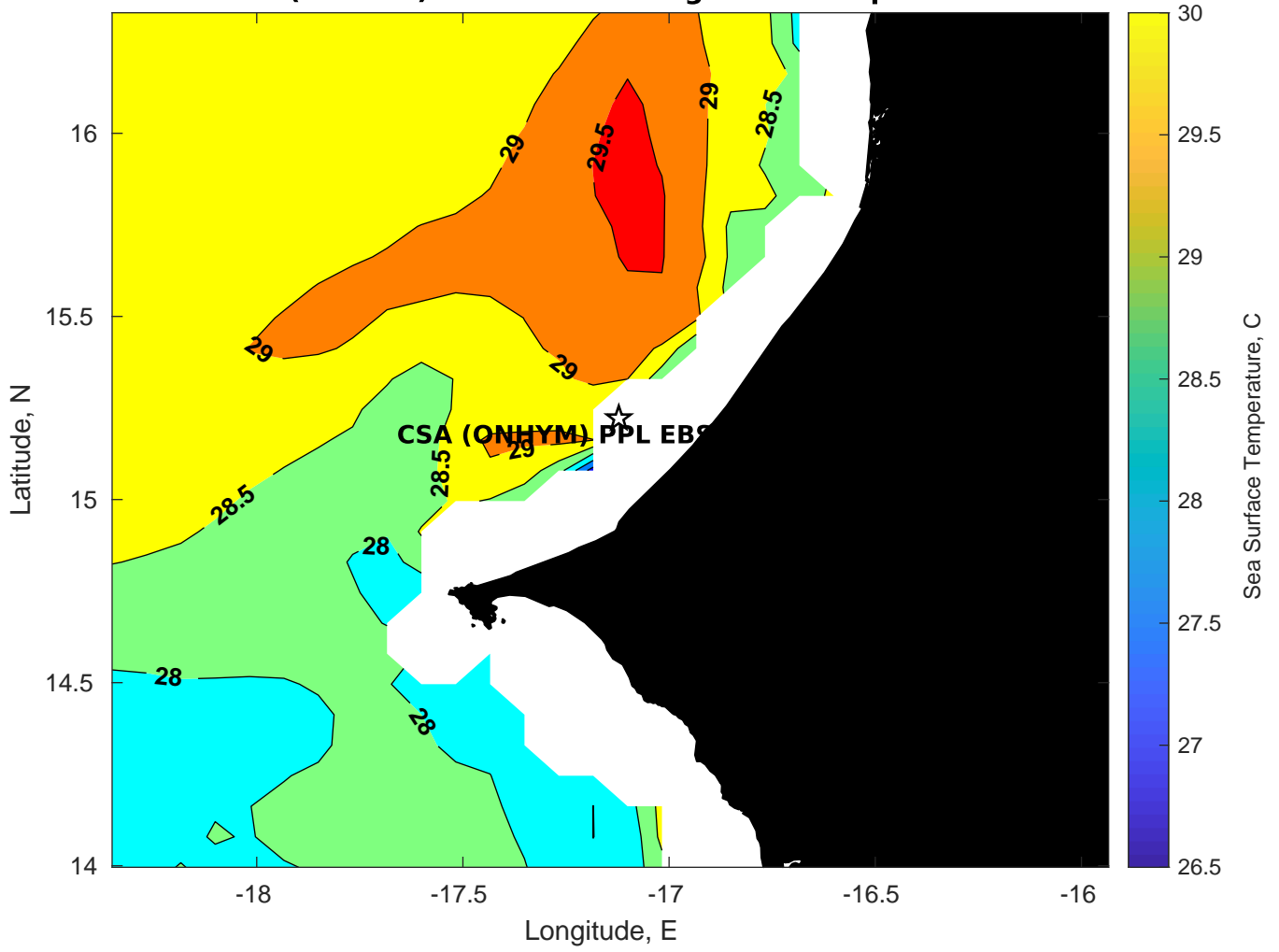
SST for CSA (ONHYM) PPL EBS - Senegal at 17-Sep-2025 00:00:00
