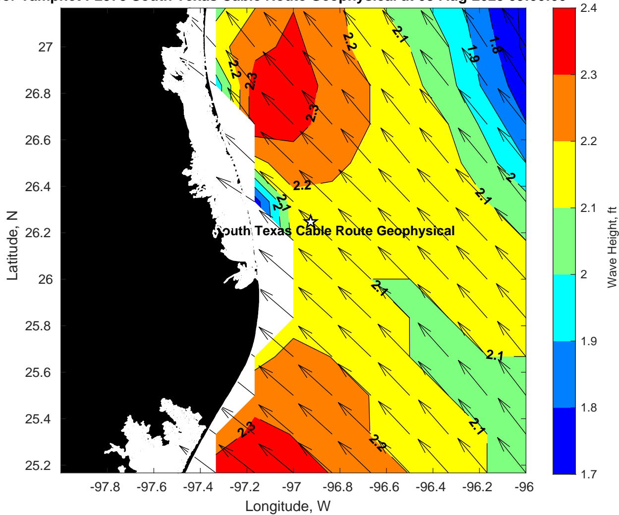
Wave Height (ft) for Tampnet P2378 South Texas Cable Route Geophysical at 08-Aug-2025 09:00:00
