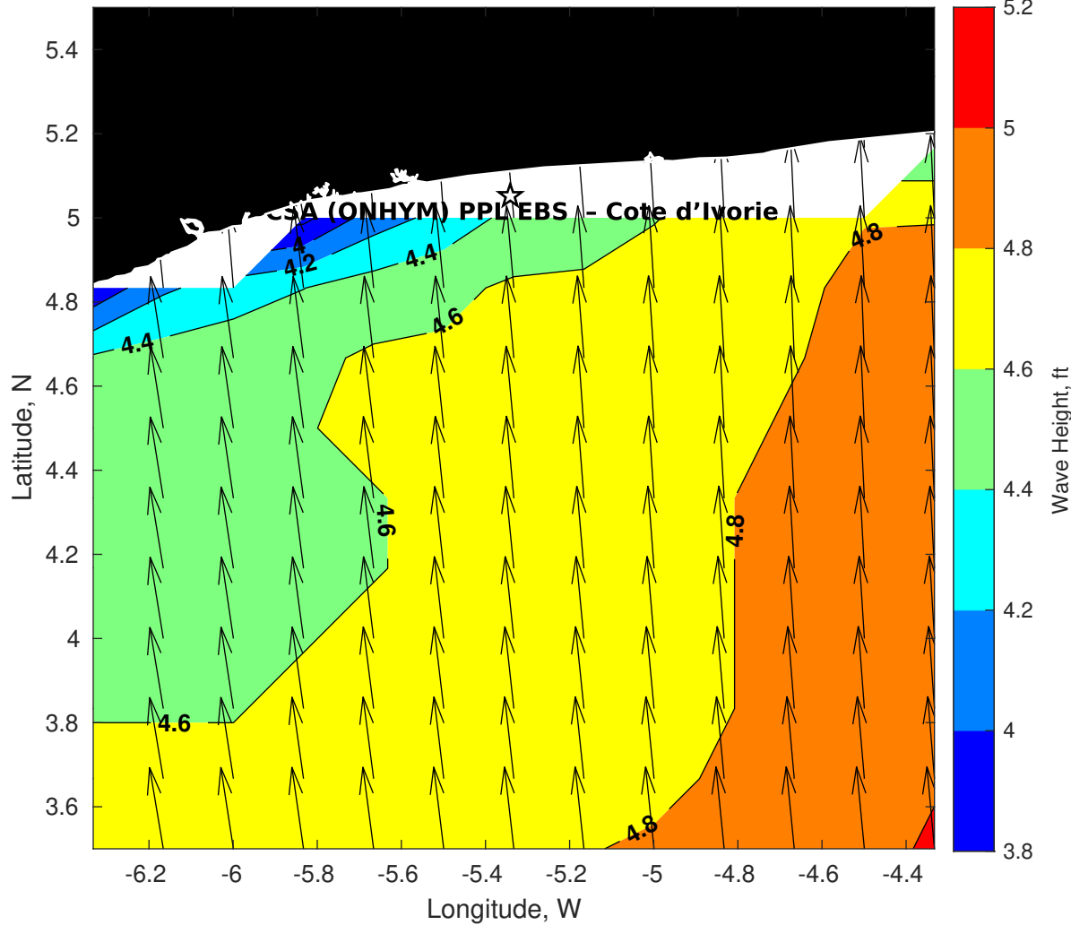
Wave Height (ft) for CSA (ONHYM) PPL EBS - Cote d'Ivoire at 25-Sep-2025 09:00:00
