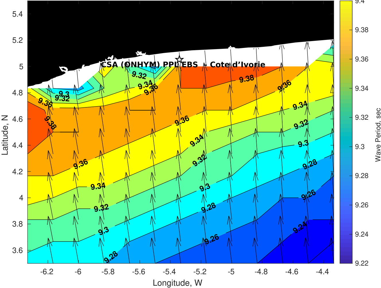
Wave Period (sec) for CSA (ONHYM) PPL EBS - Cote d'Ivoire at 25-Sep-2025 09:00:00
