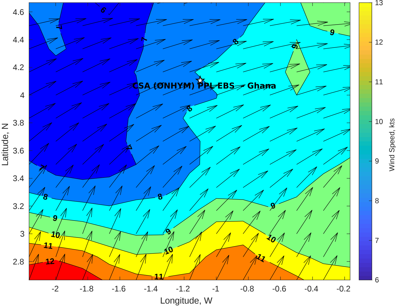
Winds (kts) for CSA (ONHYM) PPL EBS - Ghana at 25-Sep-2025 09:00:00
