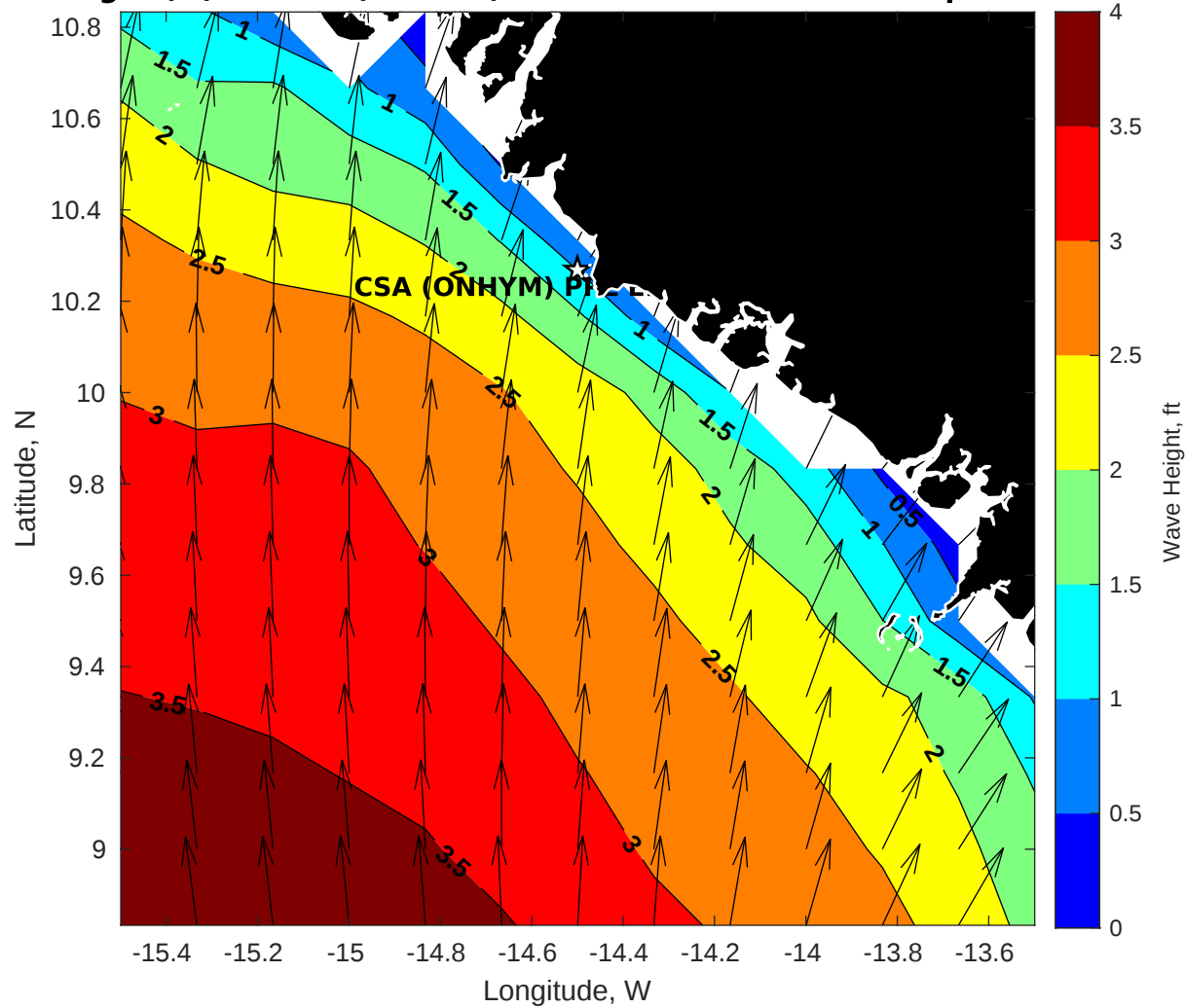
Wave Height (ft) for CSA (ONHYM) PPL EBS - Guinea at 25-Sep-2025 09:00:00
