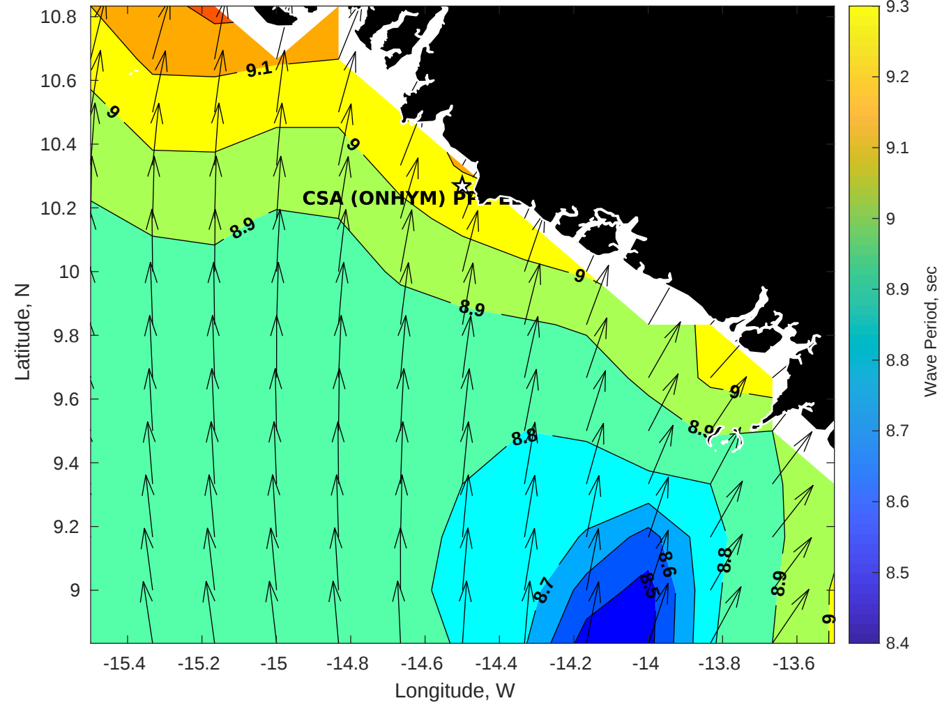
Wave Period (sec) for CSA (ONHYM) PPL EBS - Guinea at 25-Sep-2025 09:00:00
