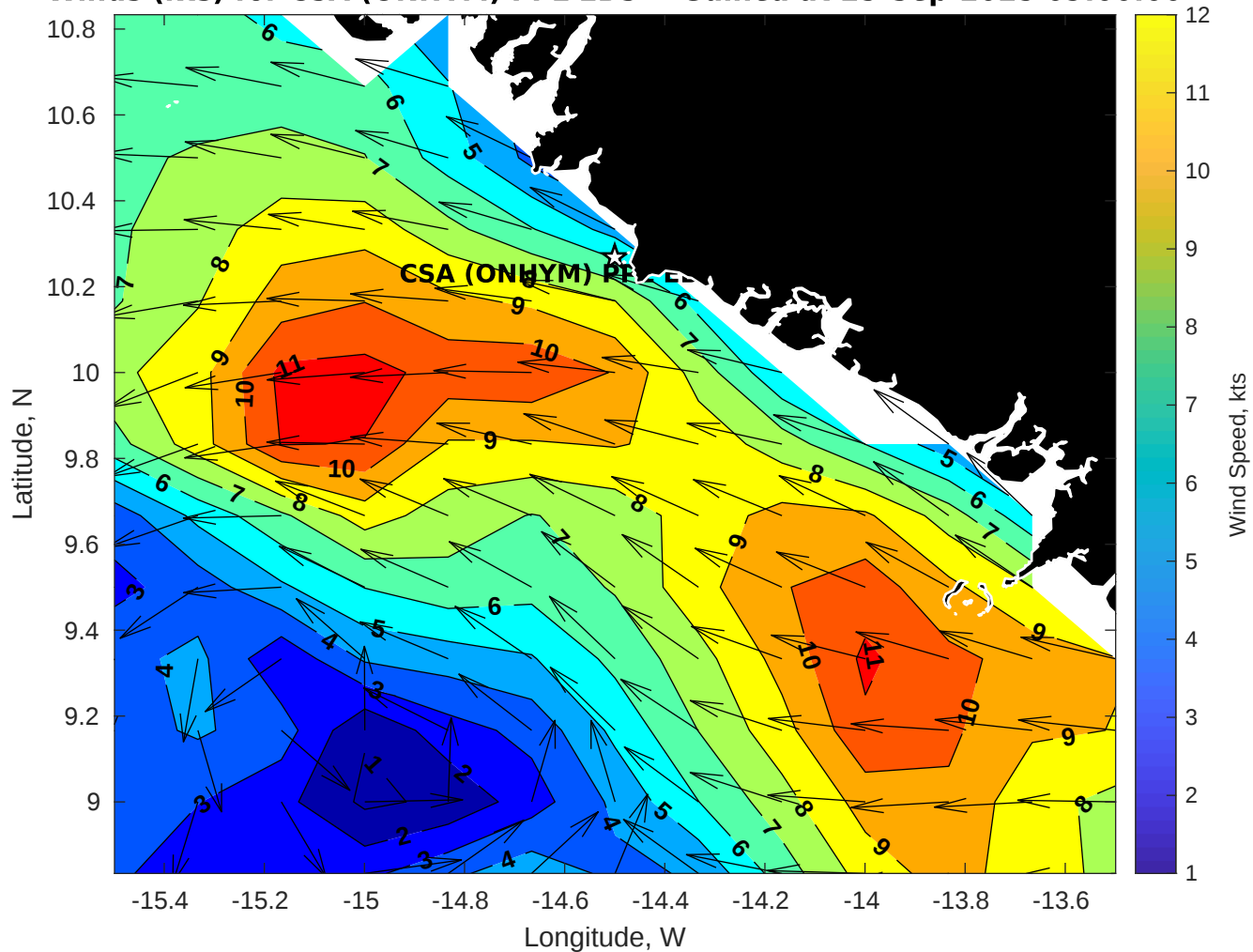
Winds (kts) for CSA (ONHYM) PPL EBS - Guinea at 25-Sep-2025 09:00:00
