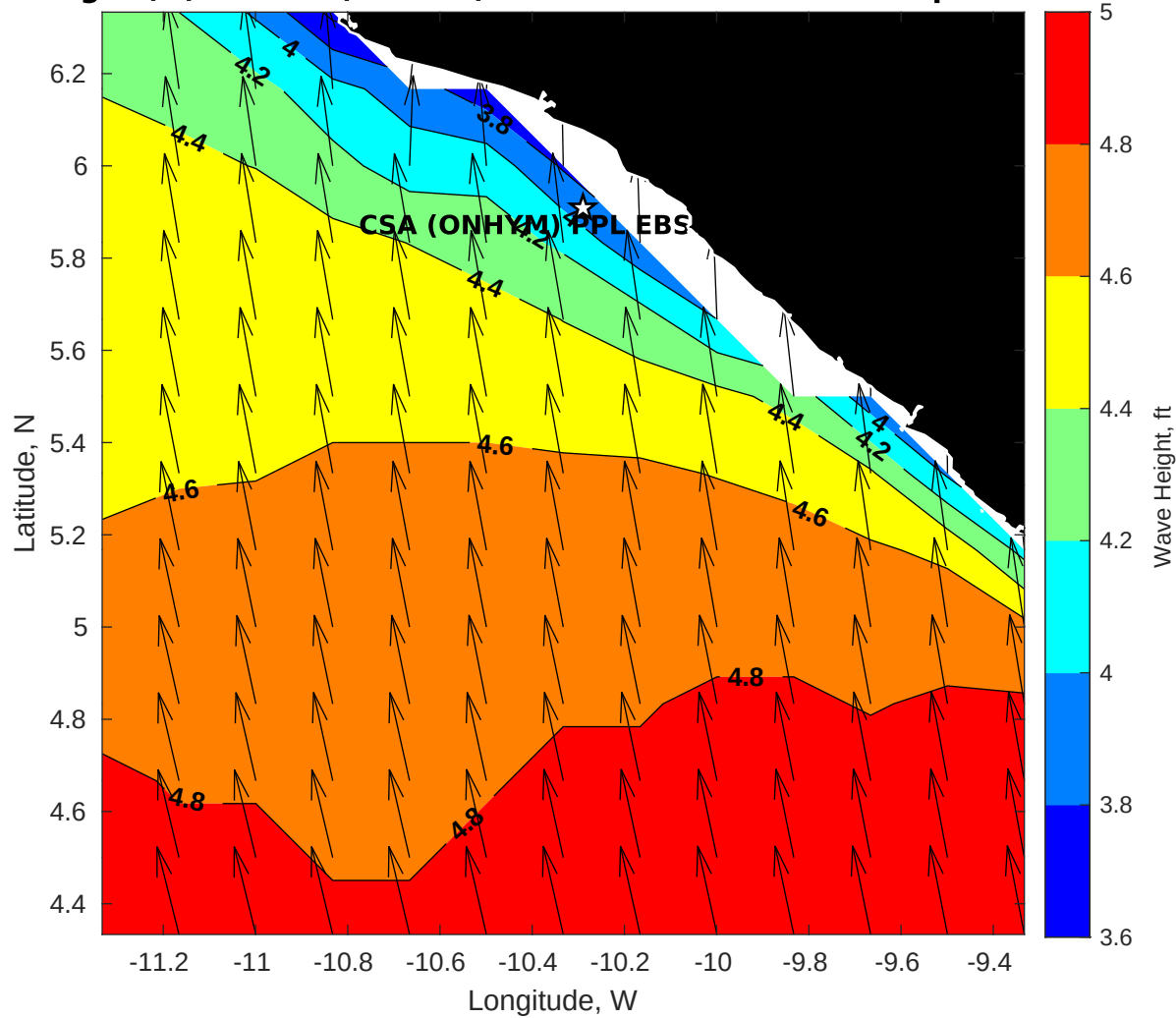
Wave Height (ft) for CSA (ONHYM) PPL EBS - Liberia at 25-Sep-2025 09:00:00
