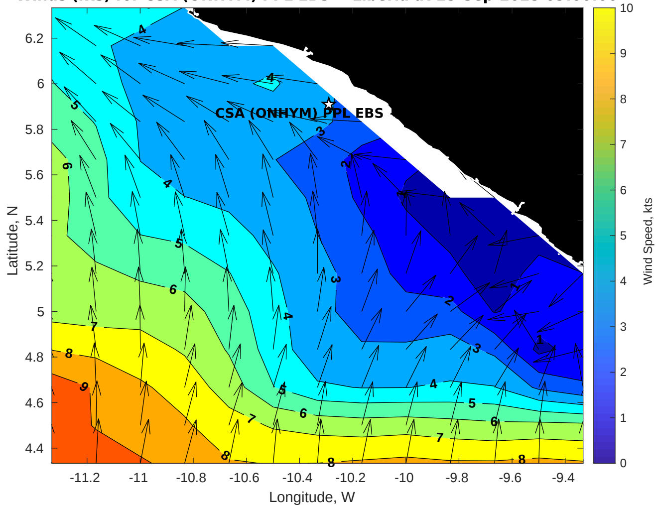
Winds (kts) for CSA (ONHYM) PPL EBS - Liberia at 25-Sep-2025 09:00:00
