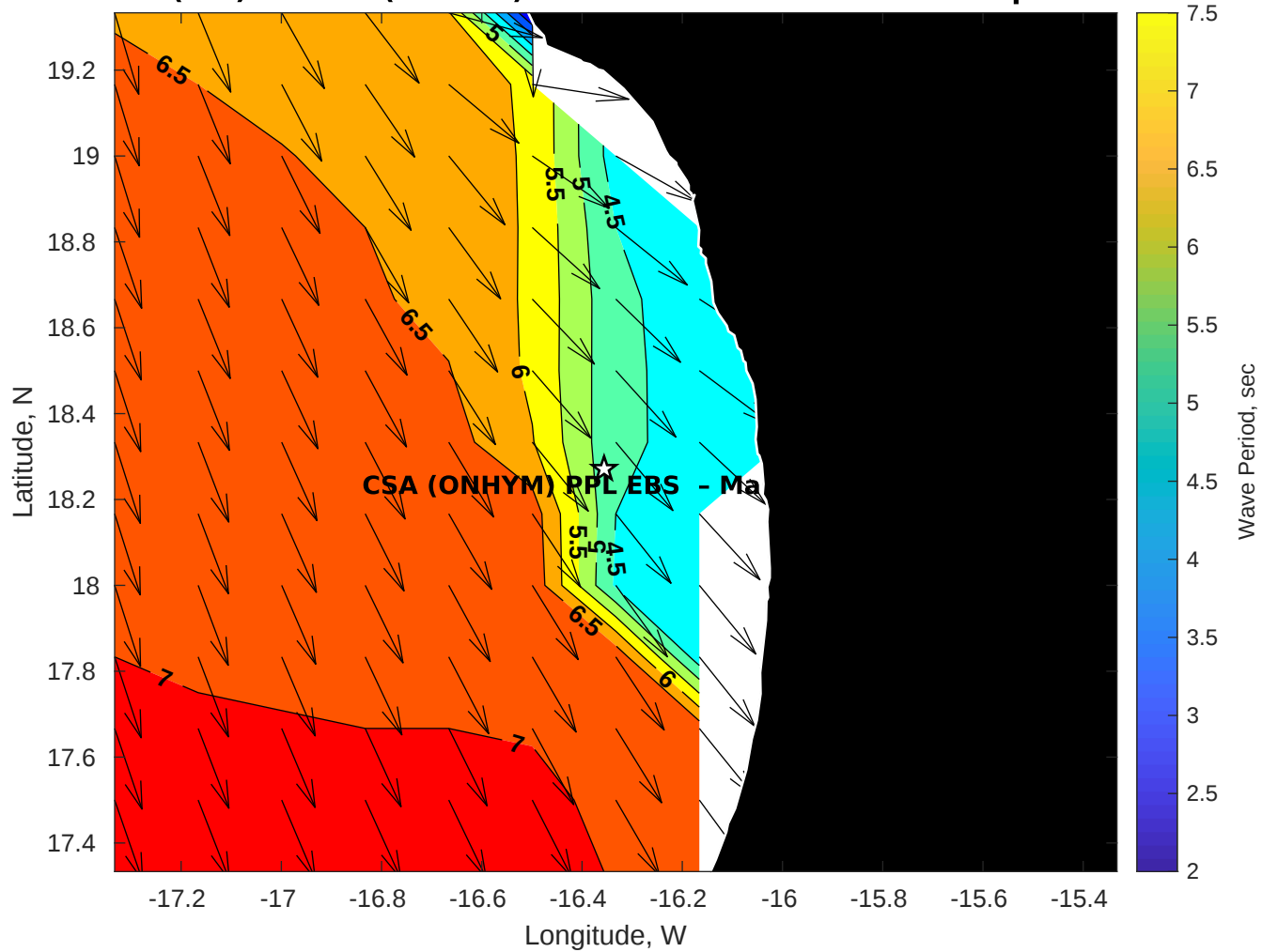
Wave Period (sec) for CSA (ONHYM) PPL EBS - Mauritania at 25-Sep-2025 09:00:00
