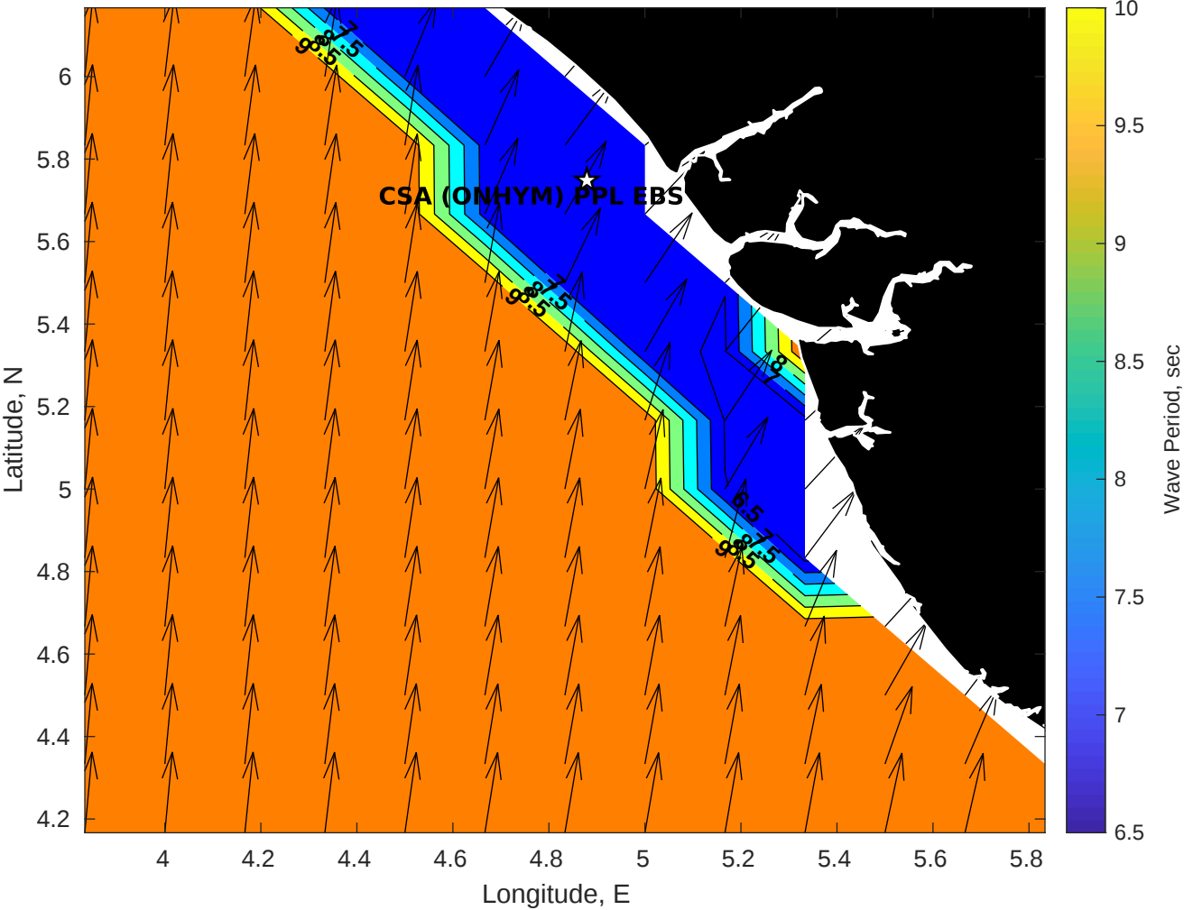
Wave Period (sec) for CSA (ONHYM) PPL EBS - Nigeria at 25-Sep-2025 09:00:00
