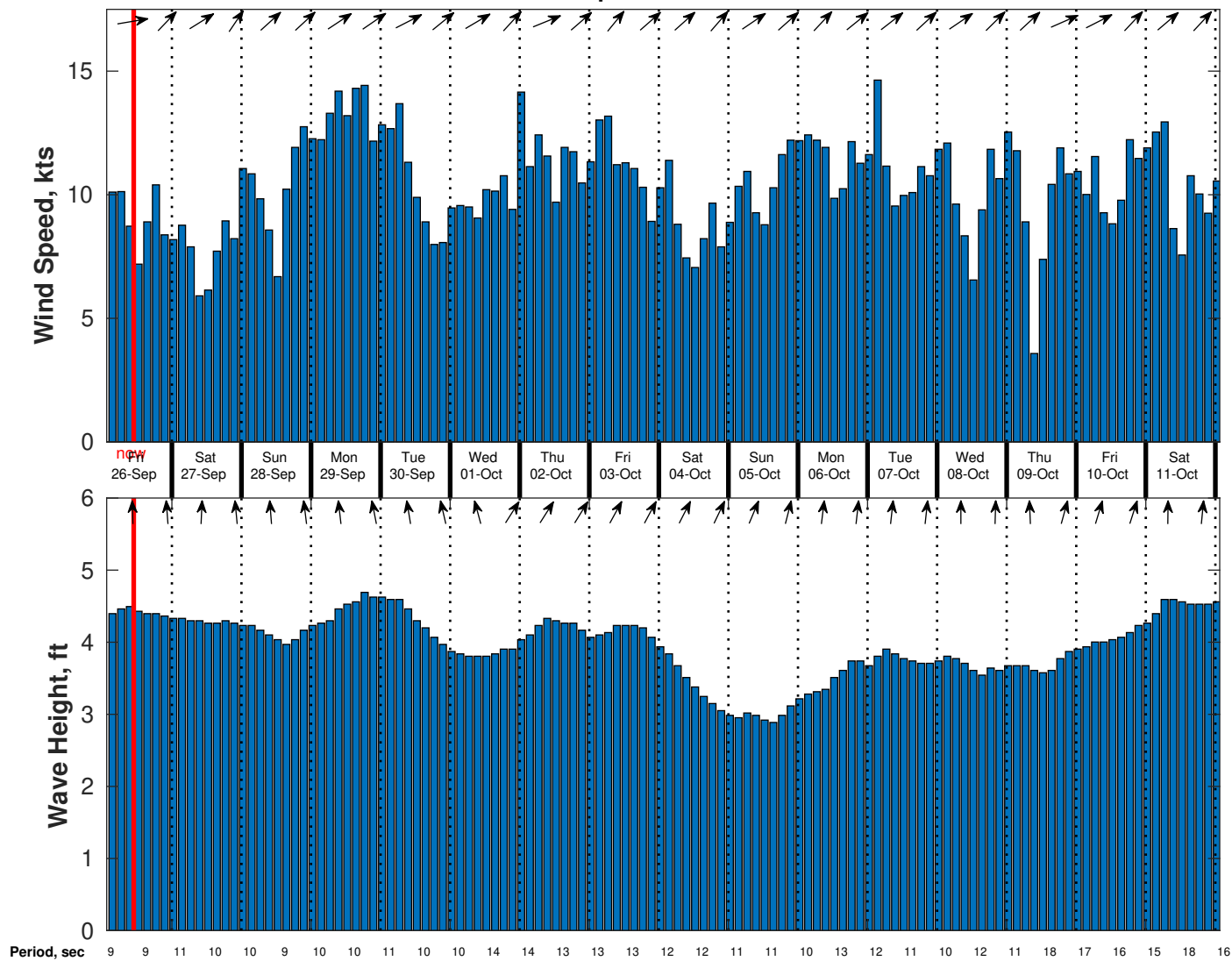
Wind & Wave Forecast for Nautilus from 25-Sep-2025 02:00:00 to 11-Oct-2025 02:00:00
