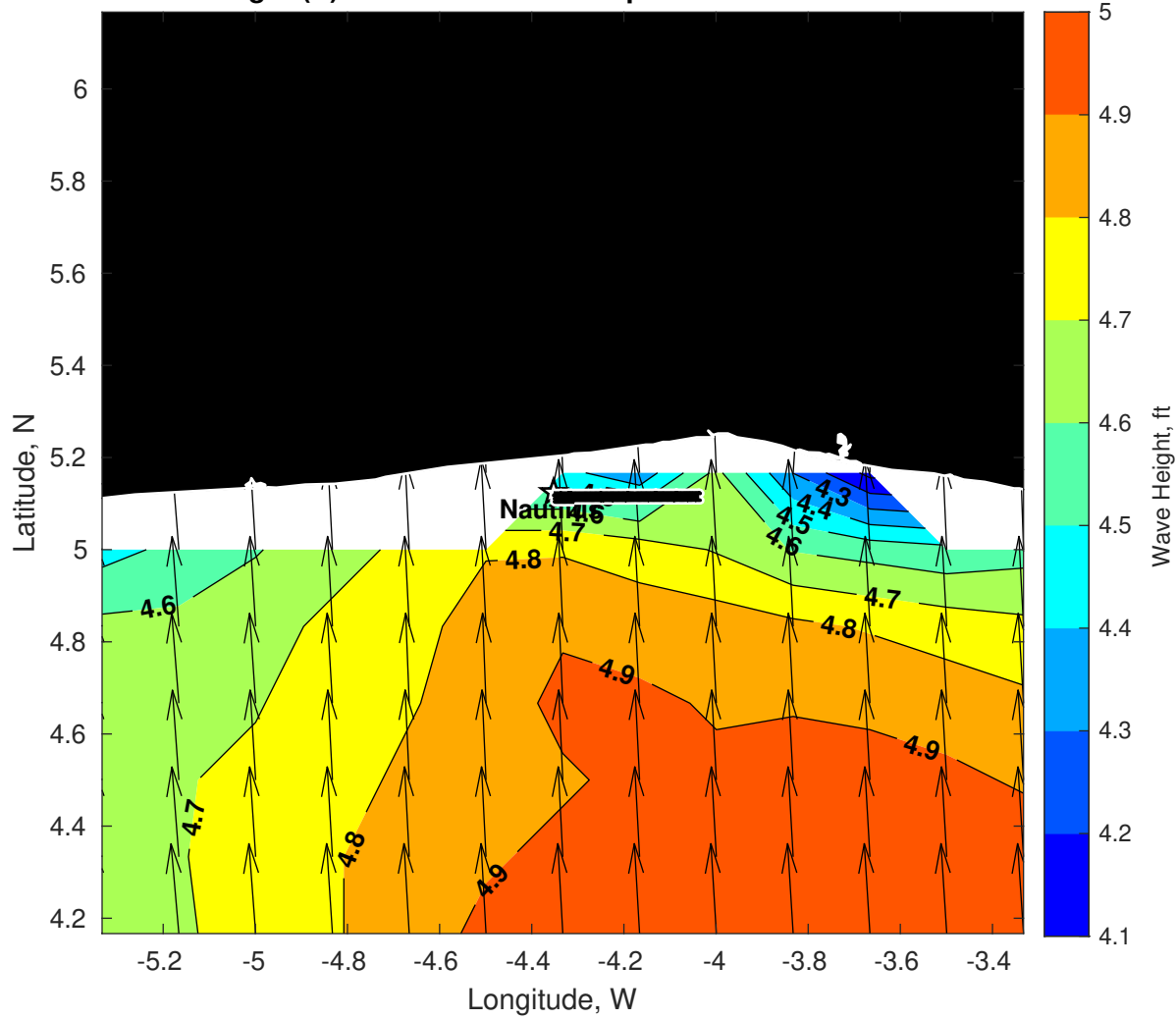
Wave Height (ft) for Nautilus at 25-Sep-2025 09:00:00
