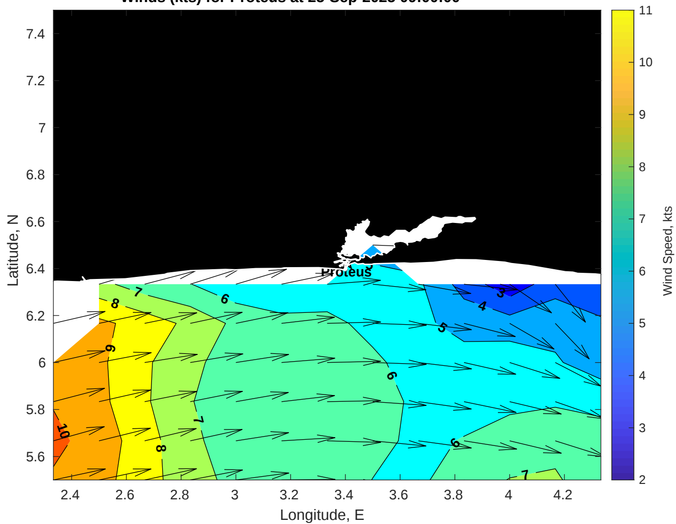
Winds (kts) for Proteus at 25-Sep-2025 09:00:00
