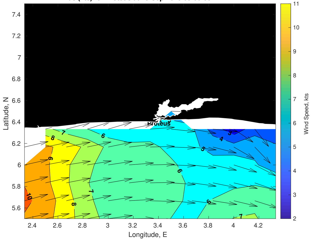
Winds (kts) for Proteus at 25-Sep-2025 09:00:00
