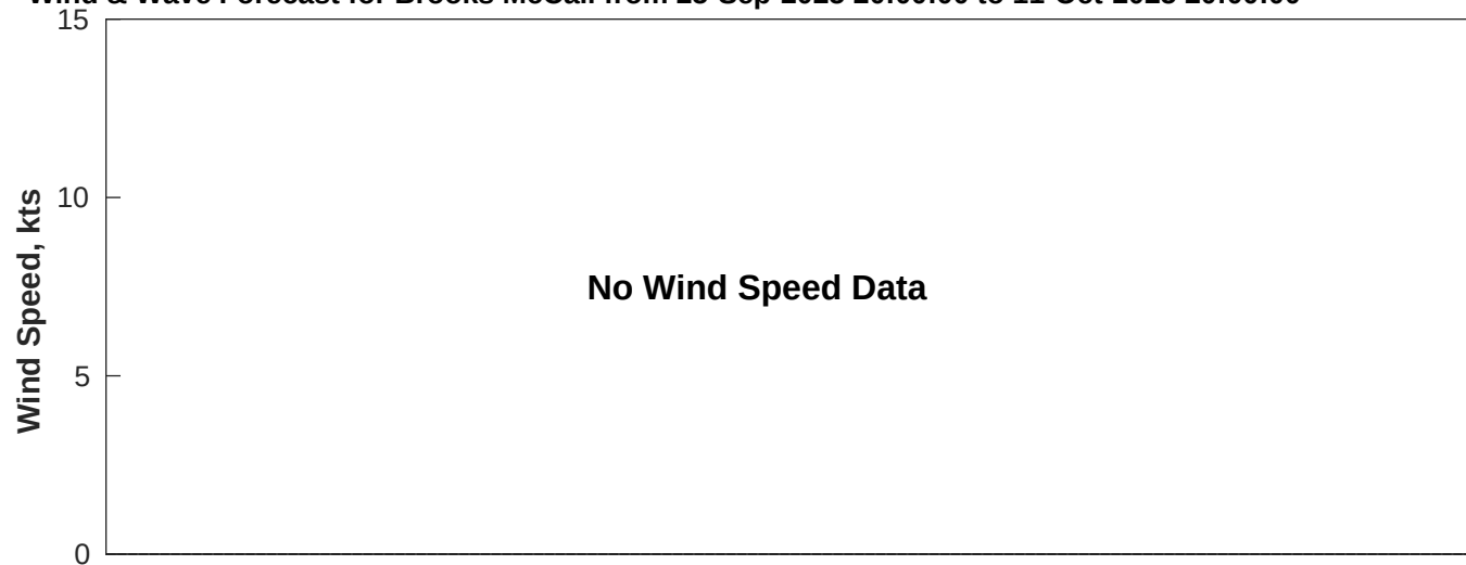
Wind & Wave Forecast for Brooks McCall from 25-Sep-2025 20:00:00 to 11-Oct-2025 20:00:00
