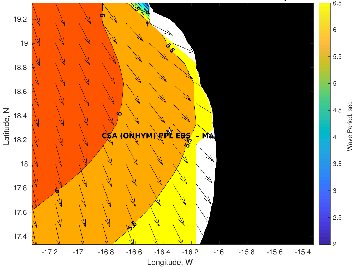
Wave Period (sec) for CSA (ONHYM) PPL EBS - Mauritania at 26-Sep-2025 09:00:00
