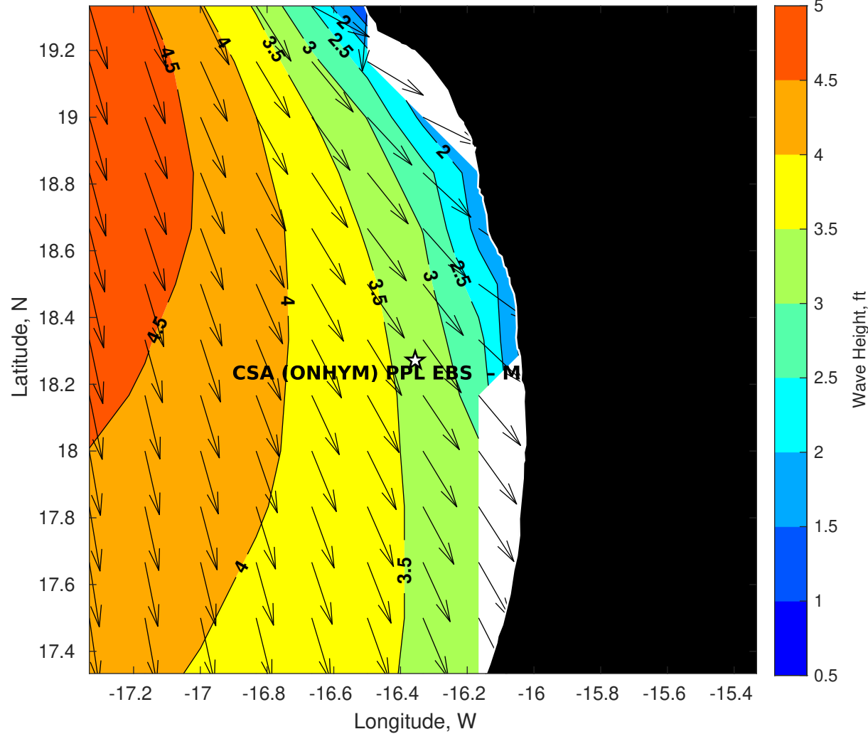
Wave Height (ft) for CSA (ONHYM) PPL EBS - Mauritania at 26-Sep-2025 09:00:00
