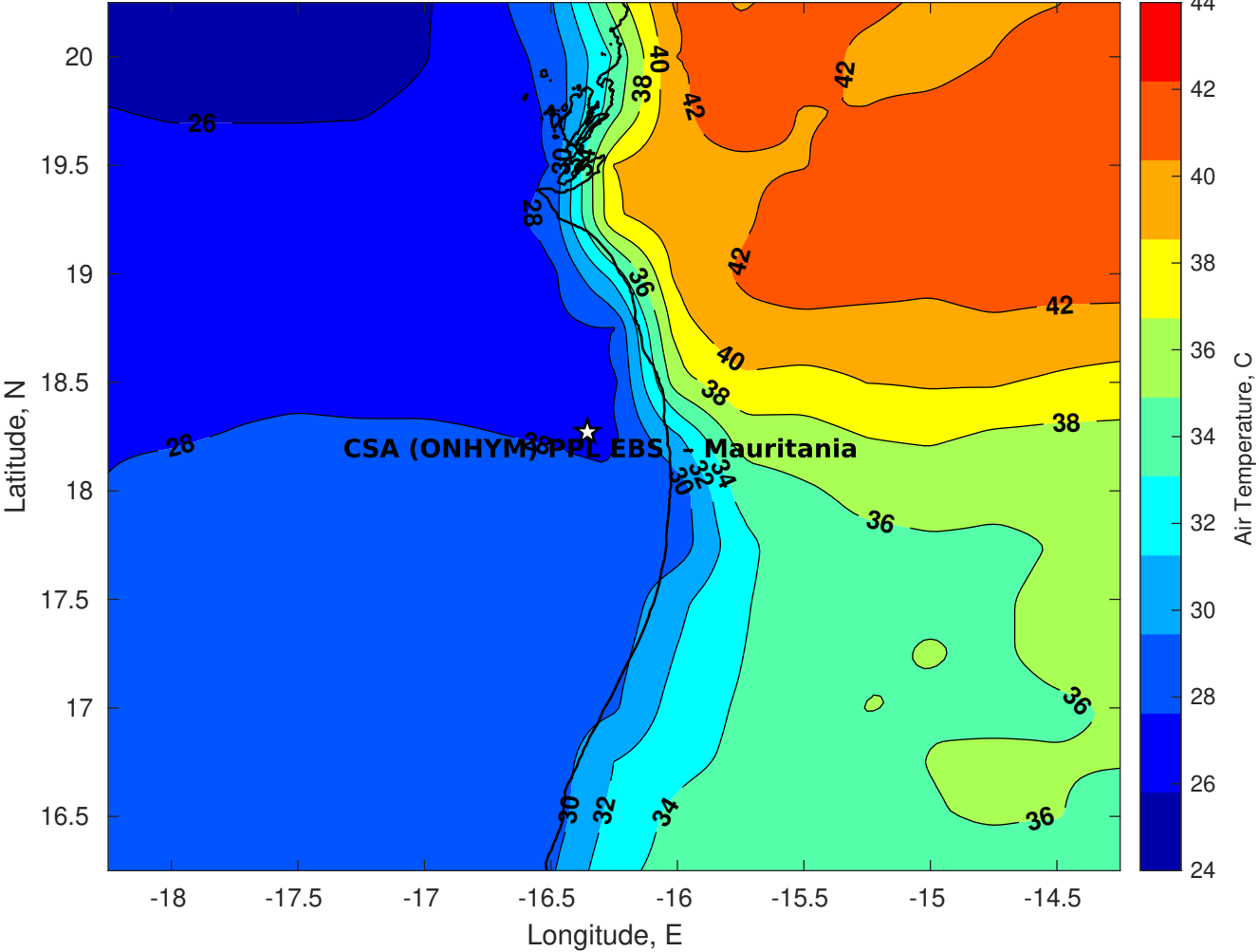
Air Temperature (C) for CSA (ONHYM) PPL EBS - Mauritania at 17-Sep-2025
