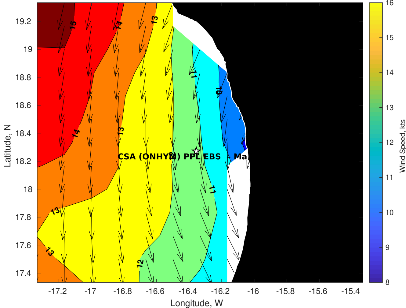
Winds (kts) for CSA (ONHYM) PPL EBS - Mauritania at 26-Sep-2025 09:00:00
