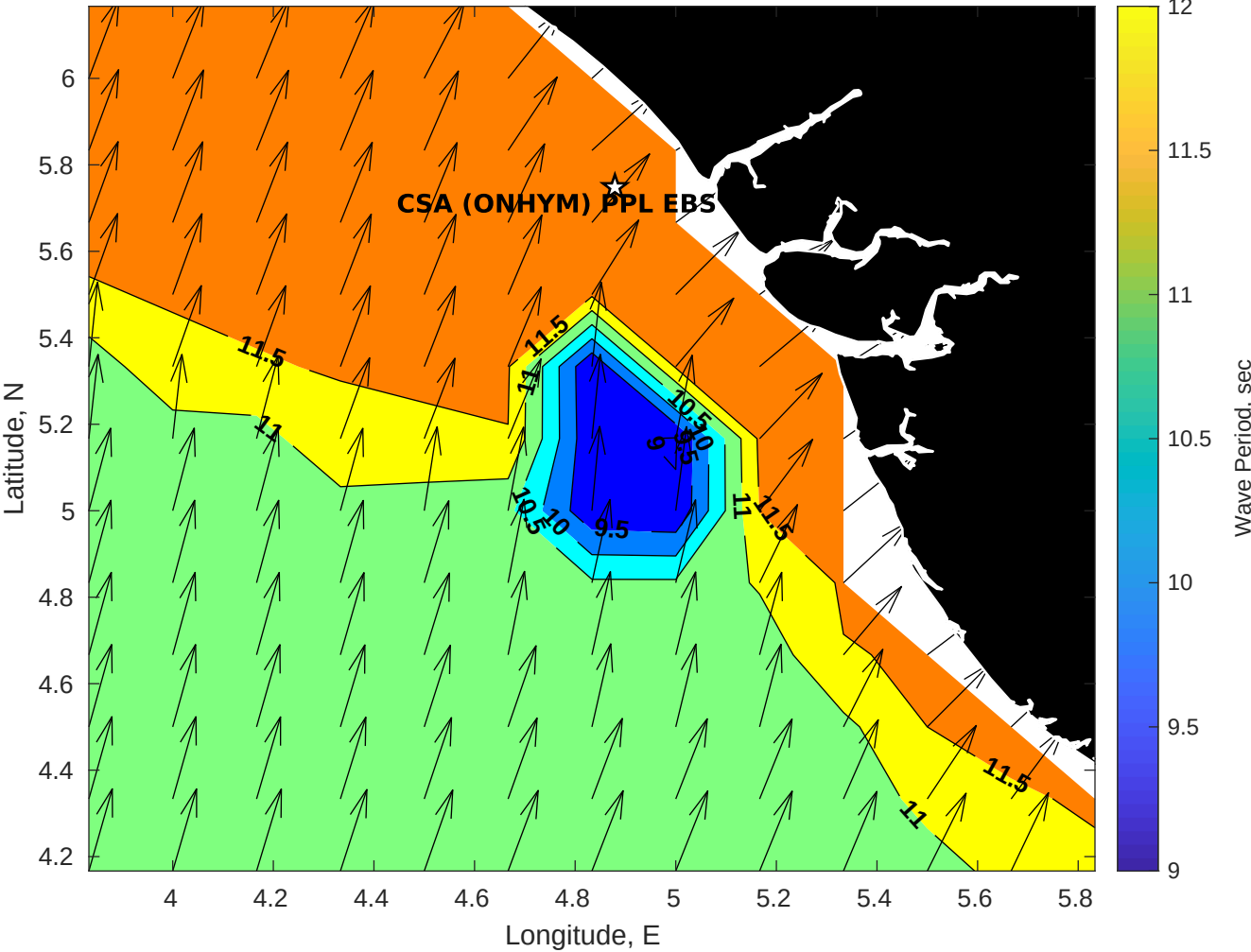
Wave Period (sec) for CSA (ONHYM) PPL EBS - Nigeria at 26-Sep-2025 09:00:00
