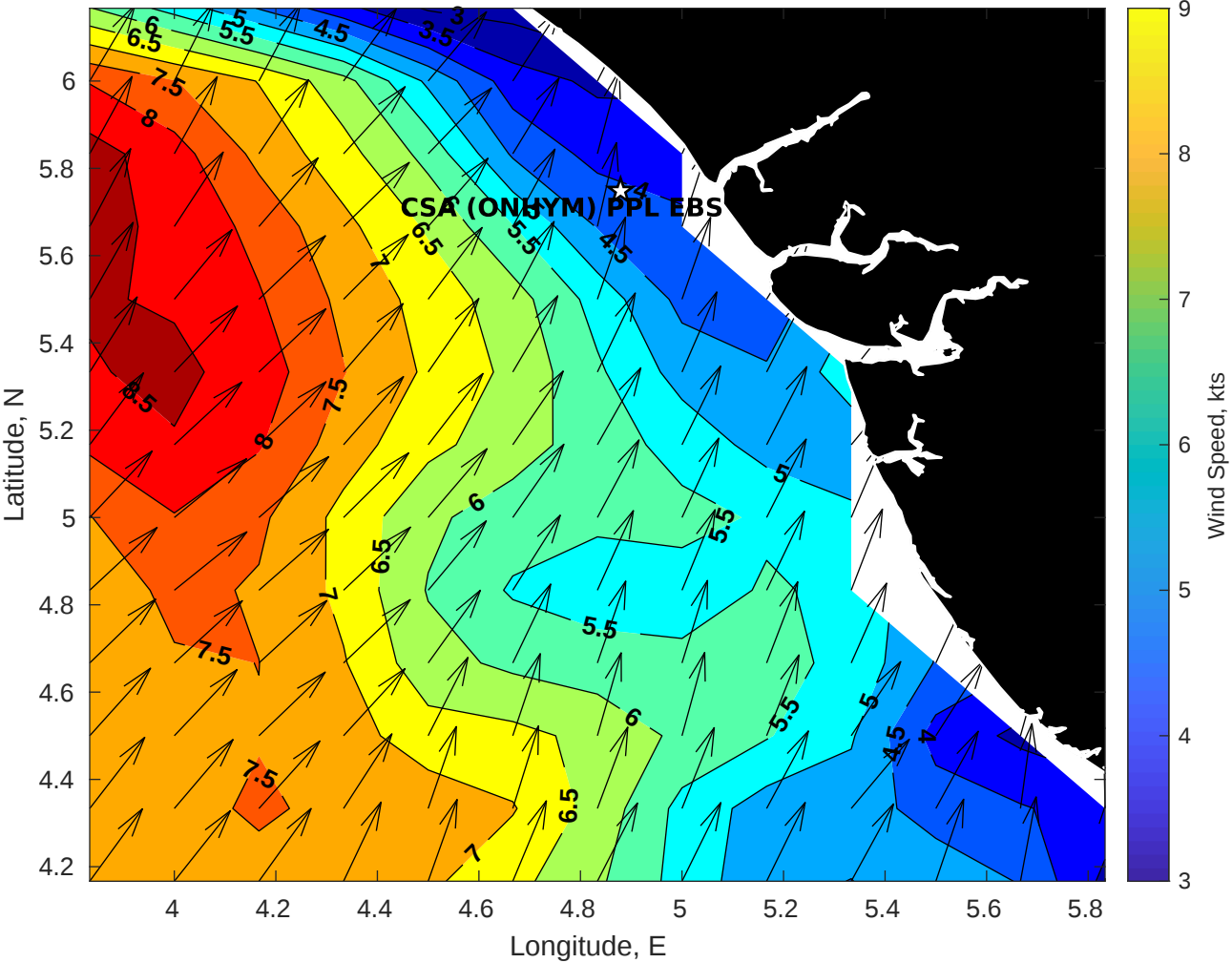
Winds (kts) for CSA (ONHYM) PPL EBS - Nigeria at 26-Sep-2025 09:00:00
