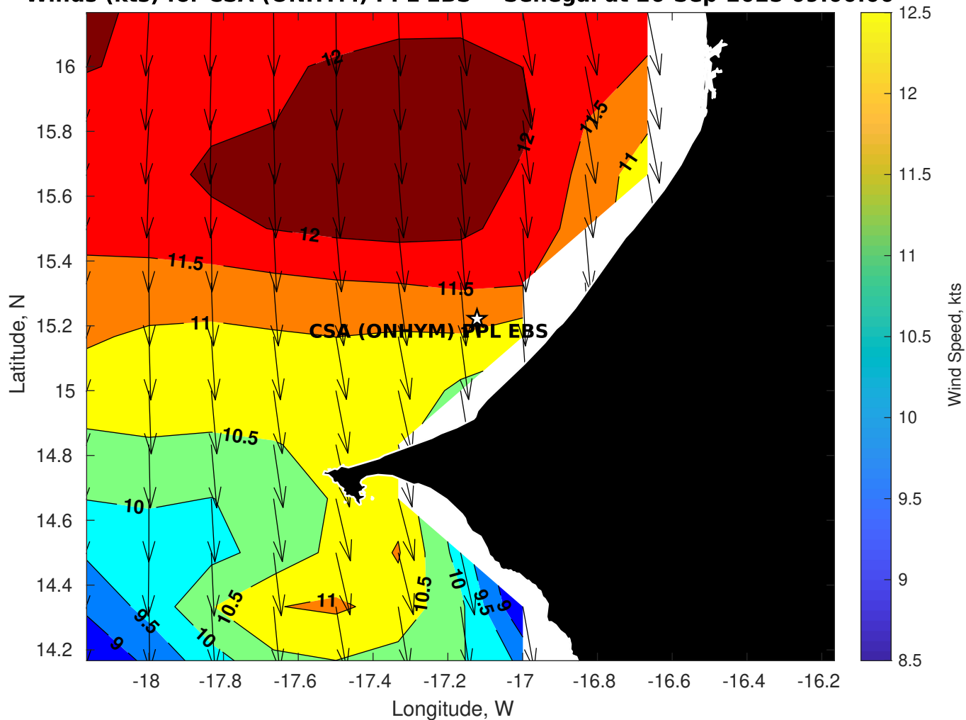
Winds (kts) for CSA (ONHYM) PPL EBS - Senegal at 26-Sep-2025 09:00:00
