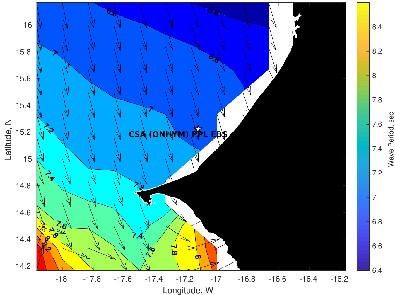
Wave Period (sec) for CSA (ONHYM) PPL EBS - Senegal at 26-Sep-2025 09:00:00
