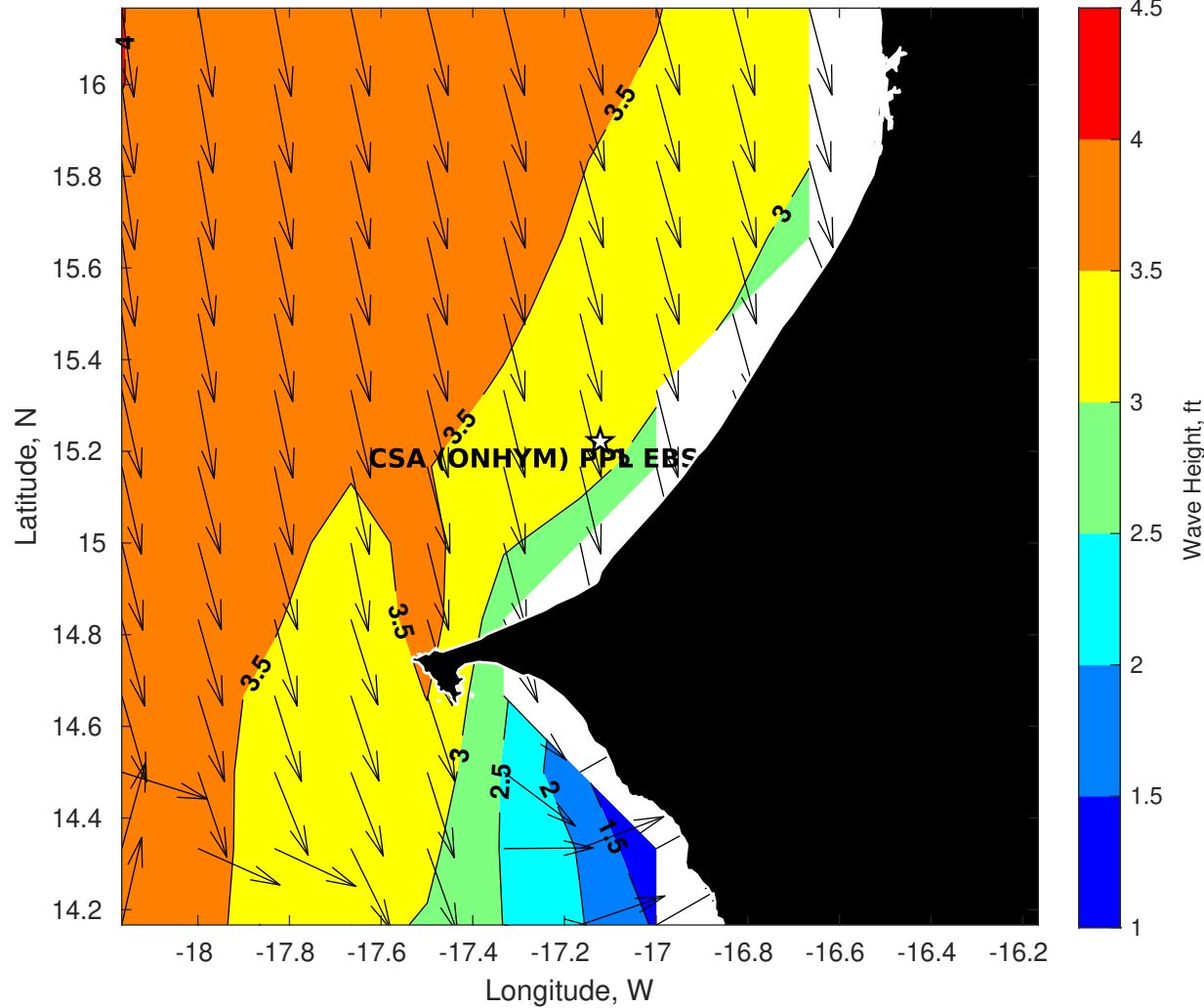
Wave Height (ft) for CSA (ONHYM) PPL EBS - Senegal at 26-Sep-2025 09:00:00
