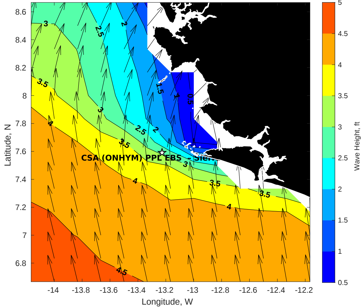
Wave Height (ft) for CSA (ONHYM) PPL EBS - Sierra Leone at 26-Sep-2025 09:00:00
