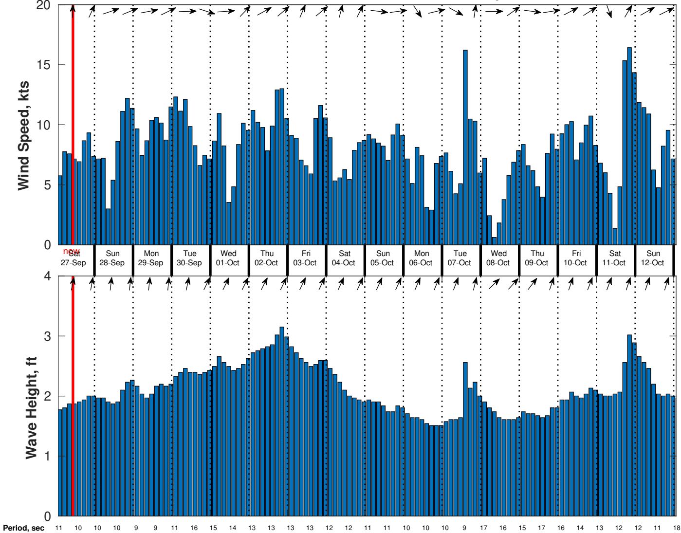
Wind & Wave Forecast for CSA (ONHYM) PPL EBS - Sierra Leone from 26-Sep-2025 01:00:00 to 12-Oct-2025 01:00:00
