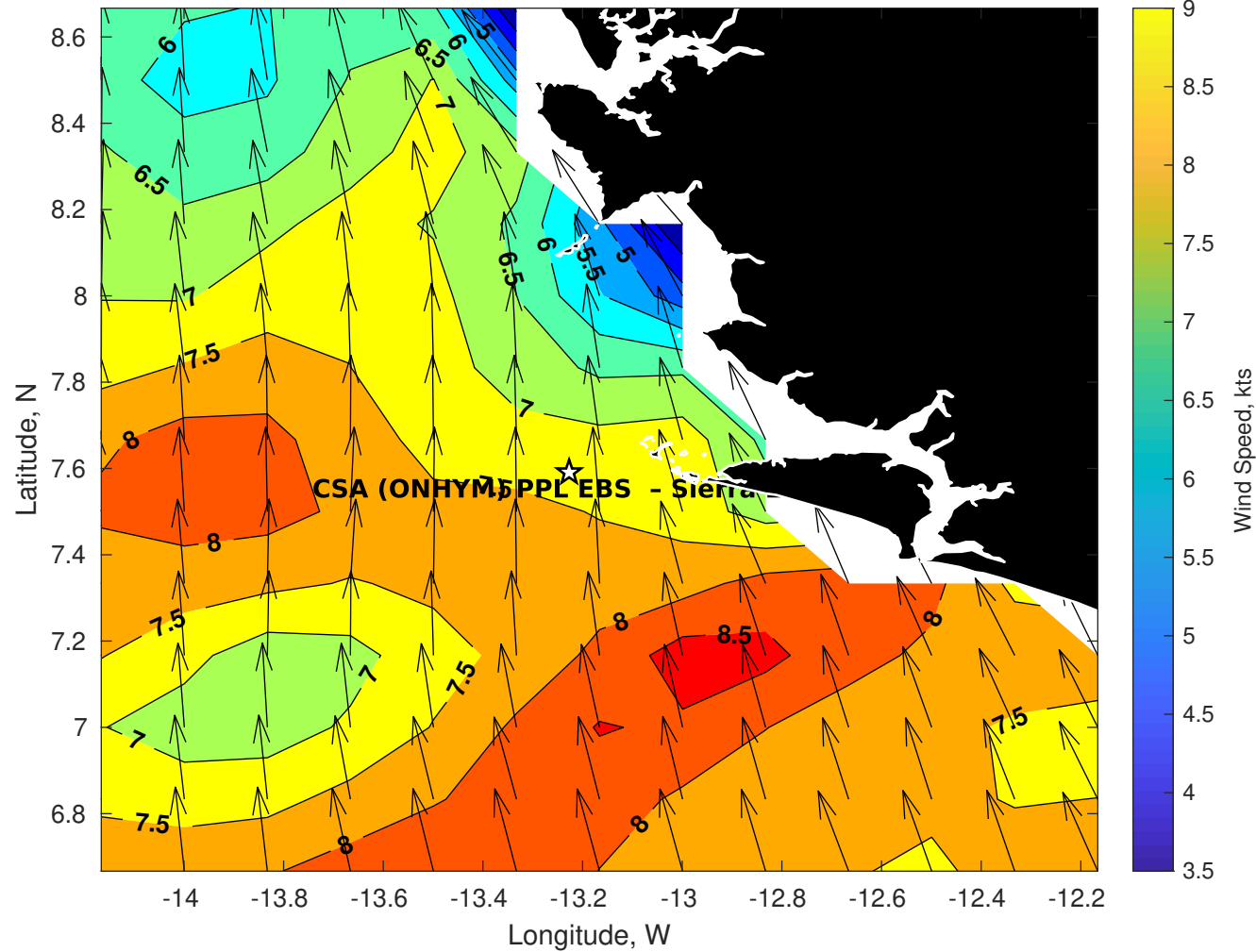
Winds (kts) for CSA (ONHYM) PPL EBS - Sierra Leone at 26-Sep-2025 09:00:00
