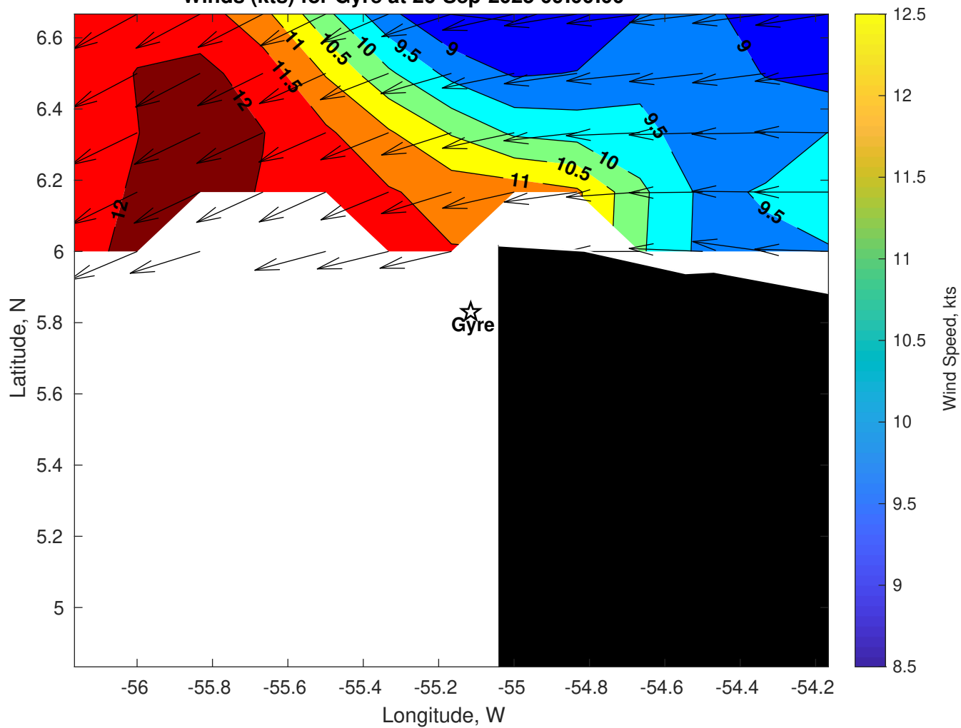
Winds (kts) for Gyre at 26-Sep-2025 09:00:00
