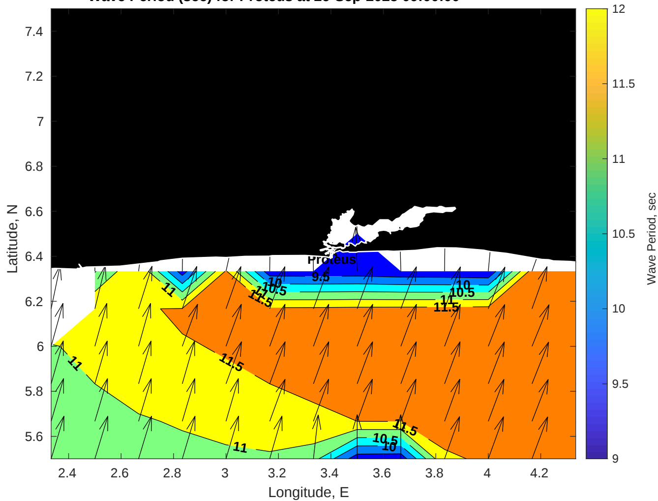
Wave Period (sec) for Proteus at 26-Sep-2025 09:00:00
