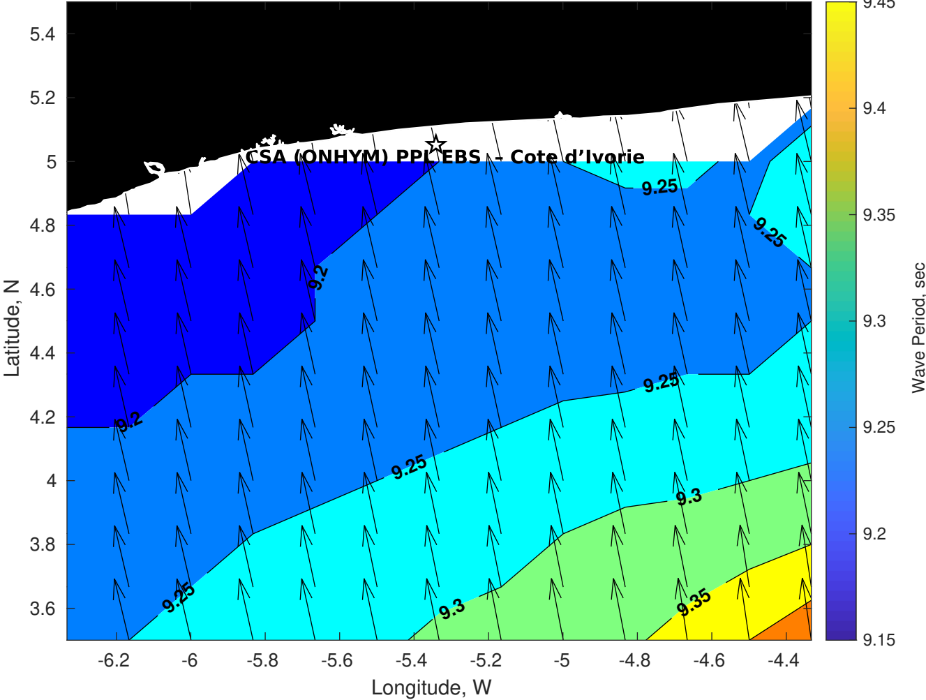
Wave Period (sec) for CSA (ONHYM) PPL EBS - Cote d'Ivoire at 27-Sep-2025 09:00:00
