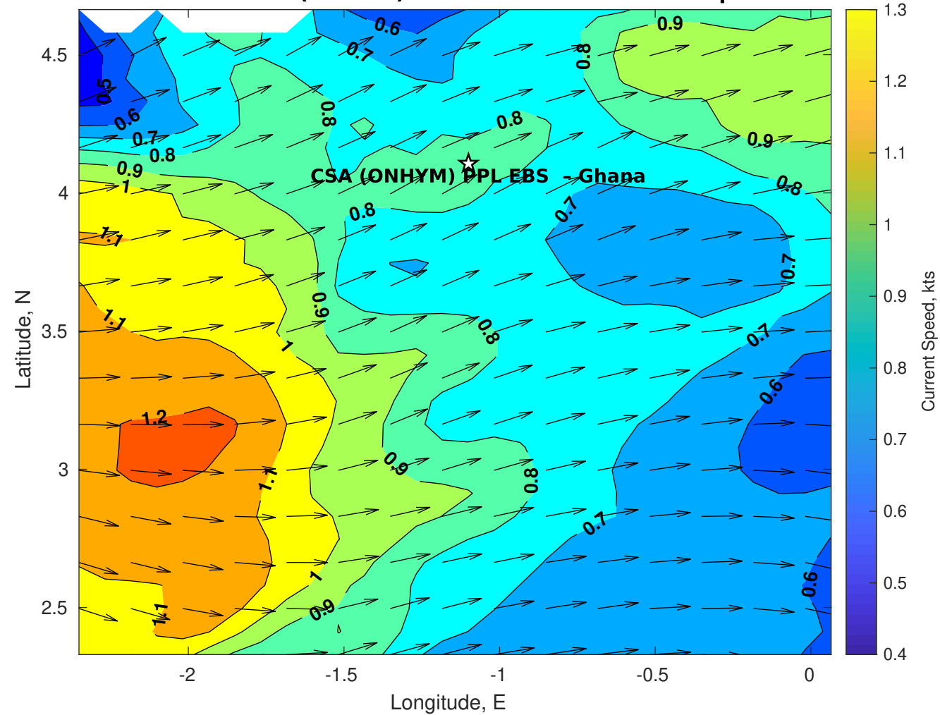
Surface Currents for CSA (ONHYM) PPL EBS - Ghana at 17-Sep-2025 00:00:00
