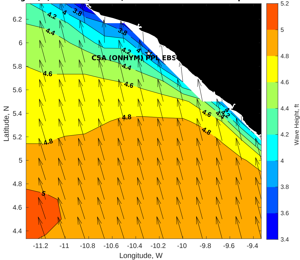
Wave Height (ft) for CSA (ONHYM) PPL EBS - Liberia at 27-Sep-2025 09:00:00
