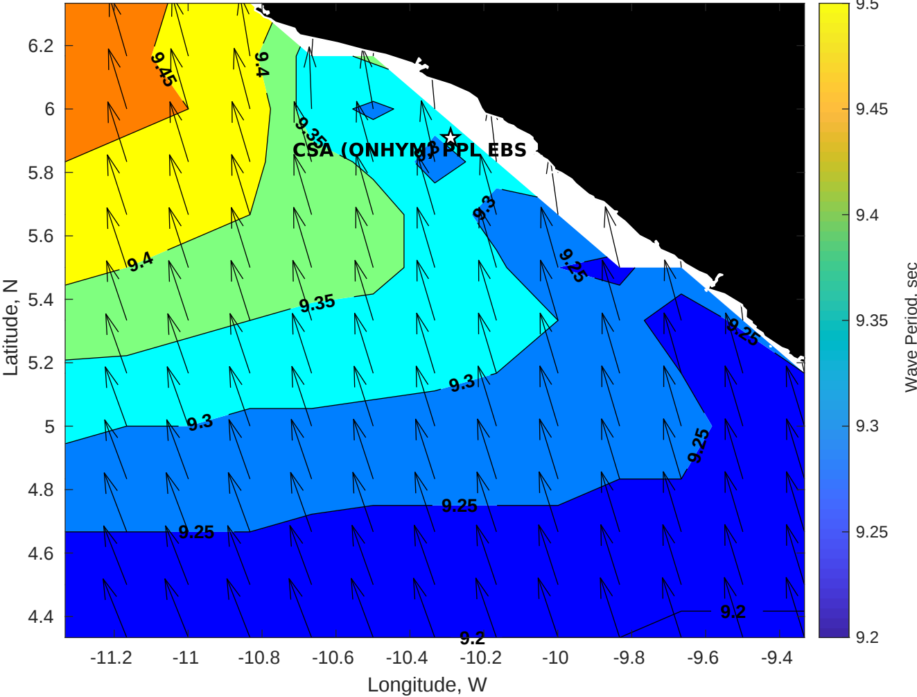
Wave Period (sec) for CSA (ONHYM) PPL EBS - Liberia at 27-Sep-2025 09:00:00
