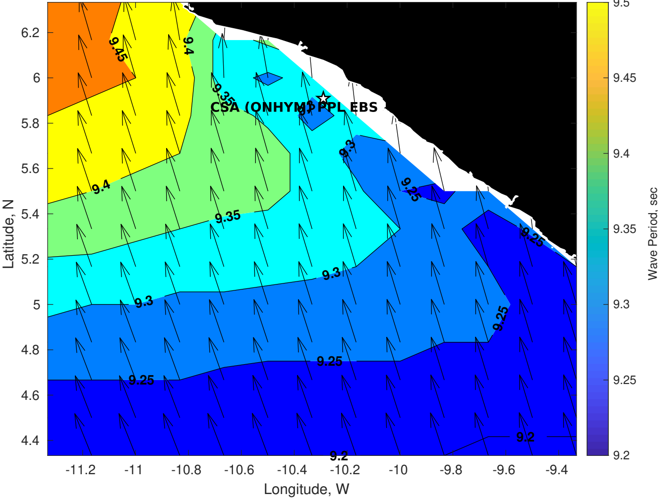
Wave Period (sec) for CSA (ONHYM) PPL EBS - Liberia at 27-Sep-2025 09:00:00
