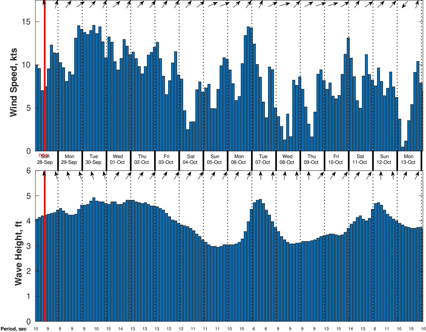
Wind & Wave Forecast for CSA (ONHYM) PPL EBS - Liberia from 27-Sep-2025 01:00:00 to 13-Oct-2025 01:00:00
