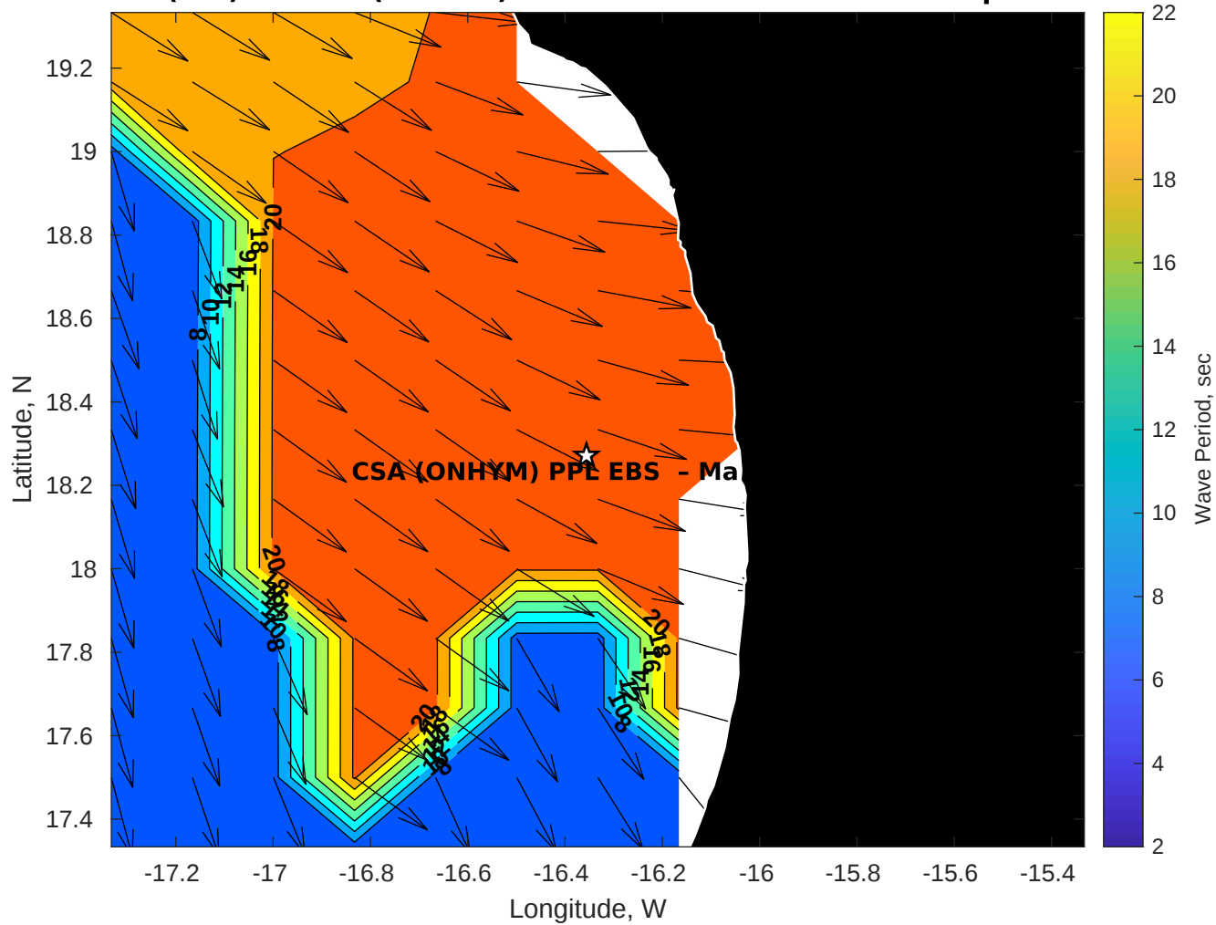
Wave Period (sec) for CSA (ONHYM) PPL EBS - Mauritania at 27-Sep-2025 09:00:00
