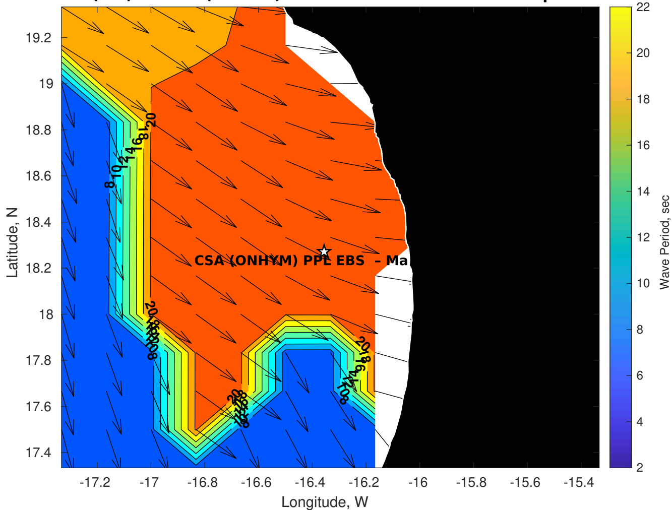
Wave Period (sec) for CSA (ONHYM) PPL EBS - Mauritania at 27-Sep-2025 09:00:00
