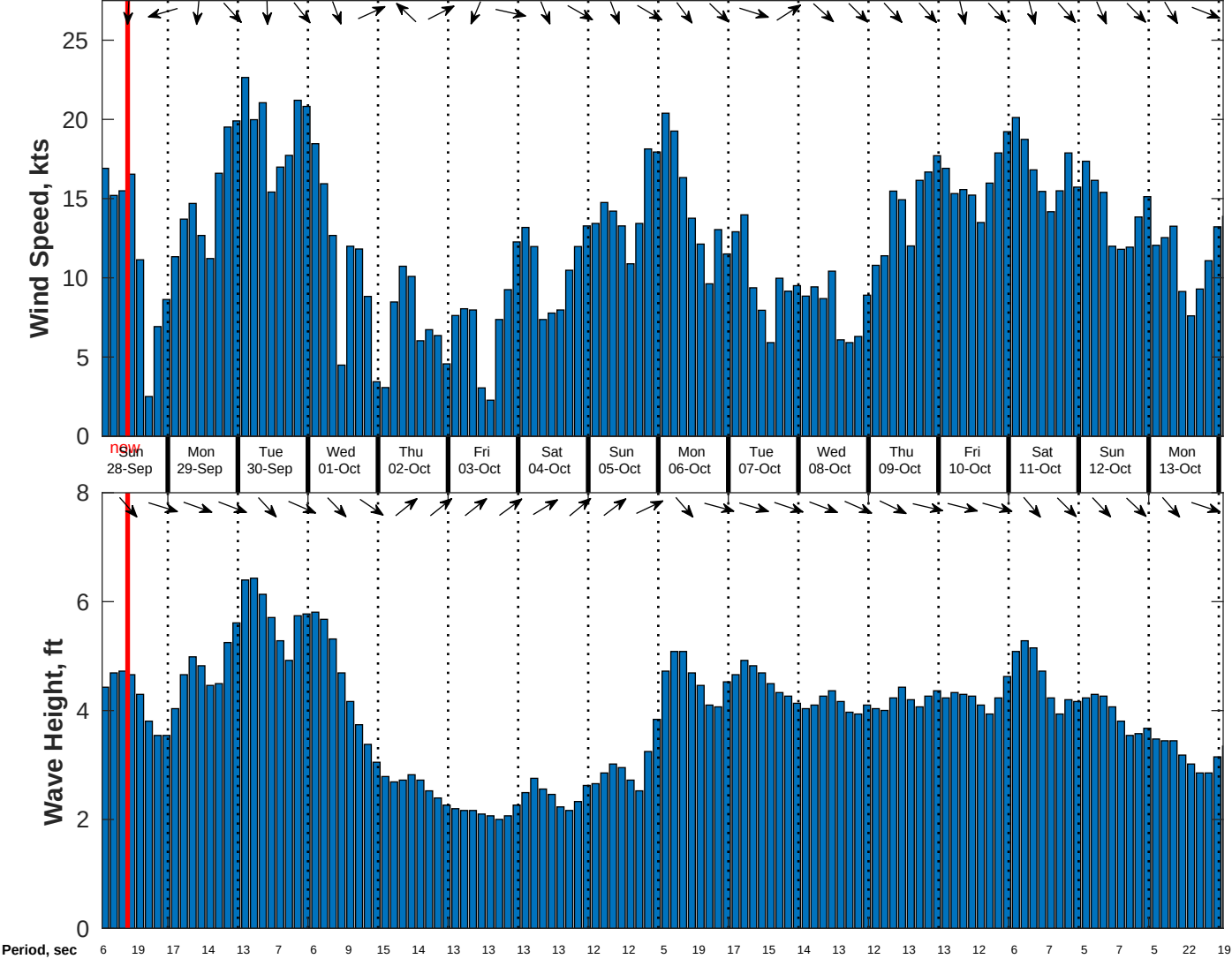
Wind & Wave Forecast for CSA (ONHYM) PPL EBS - Mauritania from 27-Sep-2025 01:00:00 to 13-Oct-2025 01:00:00
